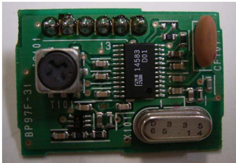
Tuner – Front without shield
