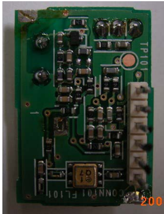
Tuner – Rear without shield
