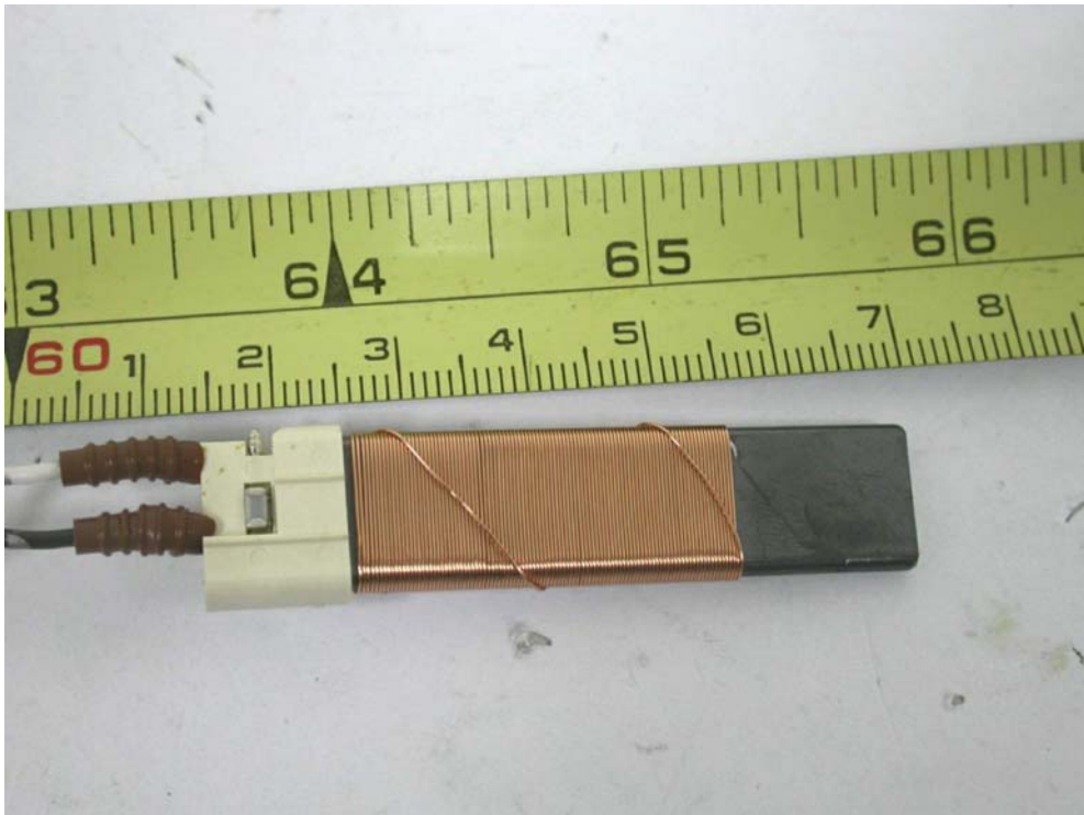
Antenna – Side B
