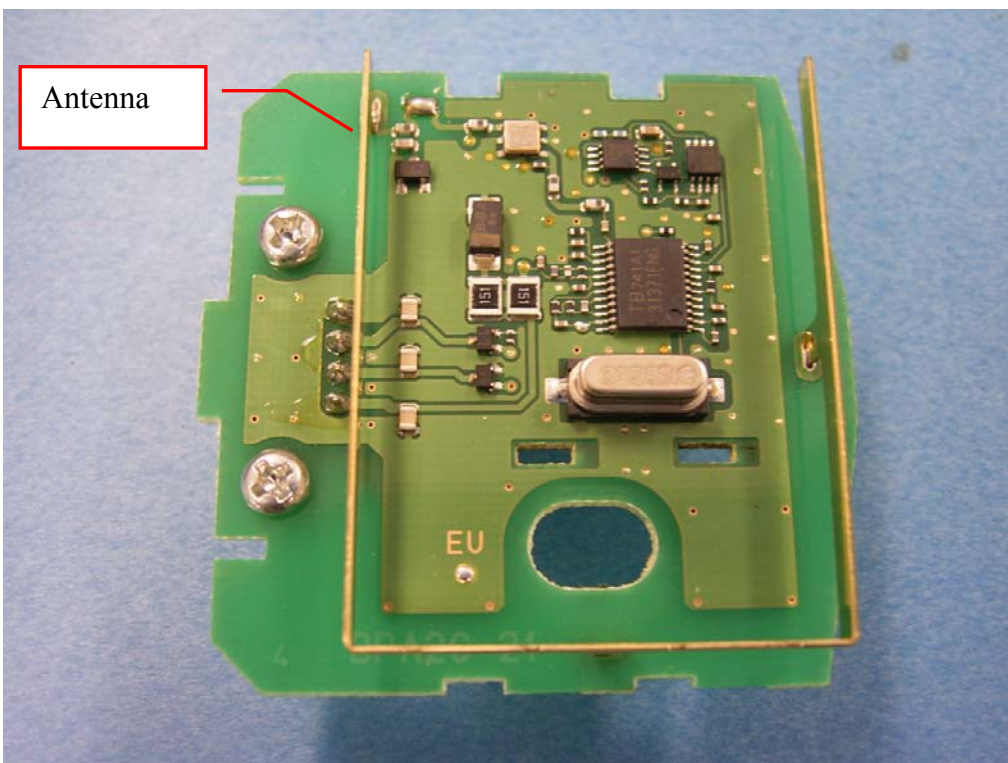
Top (without cover)
