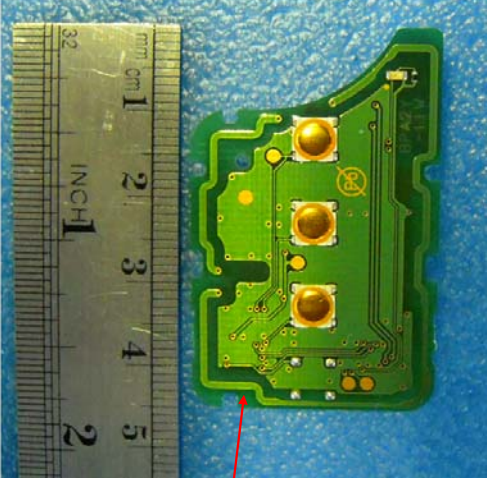
Pattern Antenna
