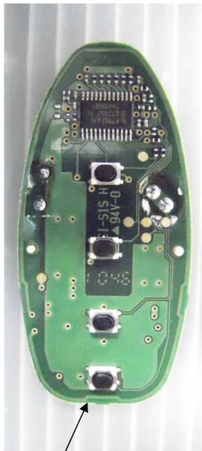
Pattern Antenna)Circumferential Pattern)
