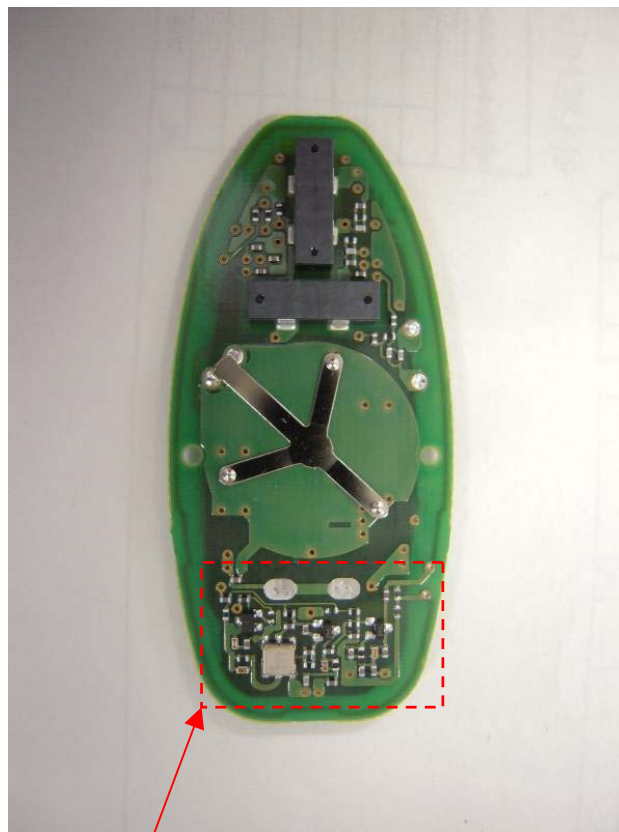
Without Shield
