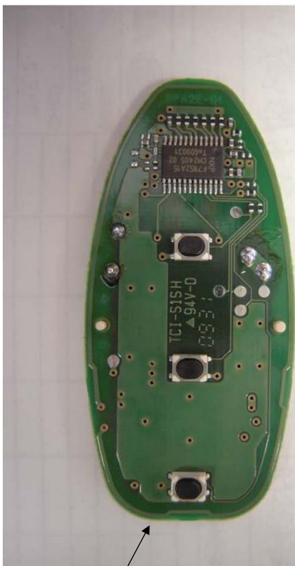
Pattern Antenna(Circumferential Pattern)
