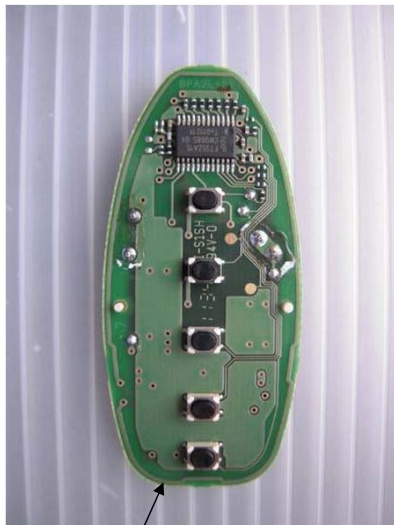
Pattern Antenna(Circumferential Pattern)
