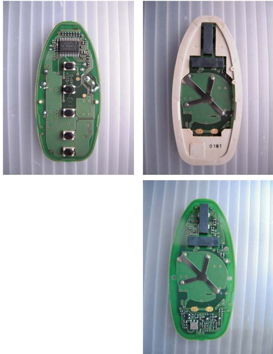
Cover Removed
