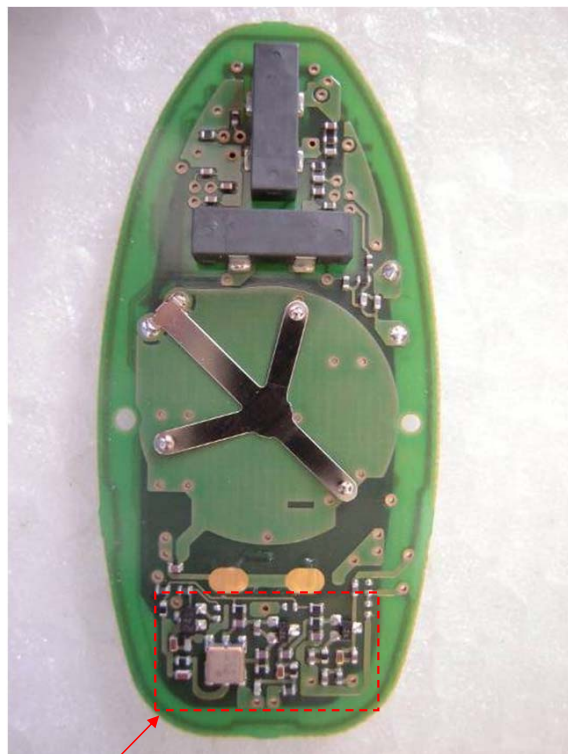
RF Circuit Part
