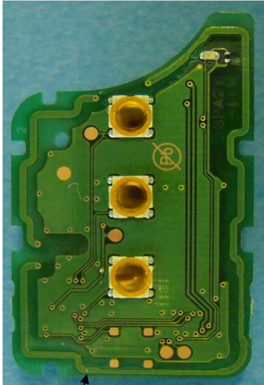
Pattern Antenna
