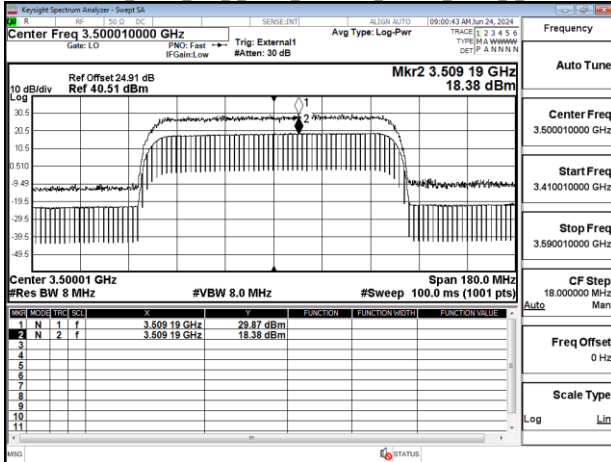
Band77-Part27 90MHz DFT s OFDM SCS30kHz 256QAM RB243 0 CH633666
