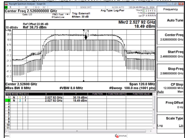
Band41 60MHz DFT s OFDM SCS30kHz 256QAM RB162 0 CH506004
