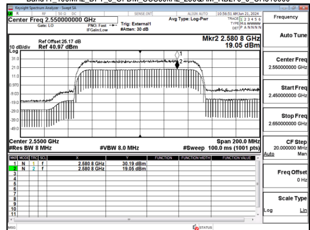
Band41 100MHz DFT s OFDM SCS30kHz 256QAM RB270 0 CH510000
