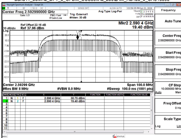
Band41 50MHz DFT s OFDM SCS30kHz 256QAM RB128 0 CH518598
