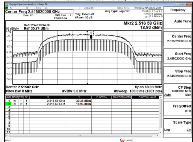
Band41 30MHz DFT s OFDM SCS30kHz 256QAM RB75_0 CH503004
