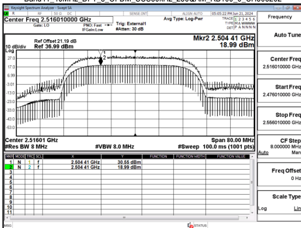
Band41 40MHz DFT s OFDM SCS30kHz 256QAM RB100 0 CH503202
