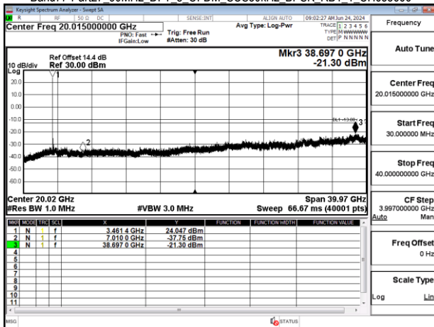
Band77-Part27_90MHz_DFT_s_OFDM_SCS30kHz_BPSK_RB1_1_CH649668
