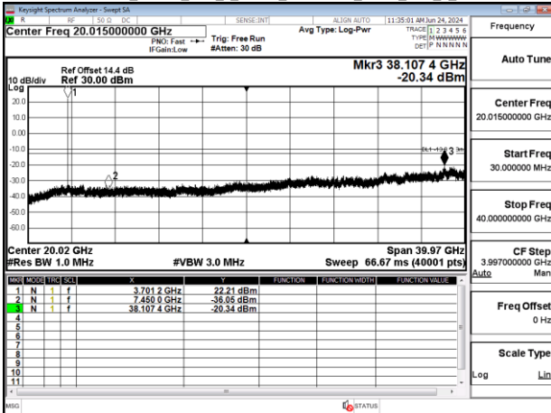
Band77-Part27_50MHz_DFT_s_OFDM_SCS30kHz_BPSK_RB1_1_CH648334
