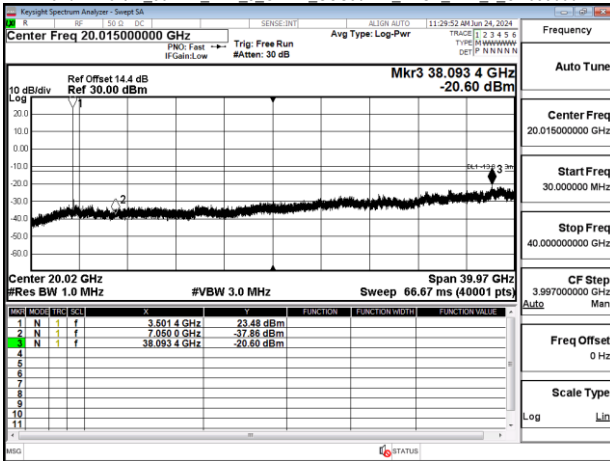
Band77-Part27_50MHz_DFT_s_OFDM_SCS30kHz_BPSK_RB1_1_CH648334
