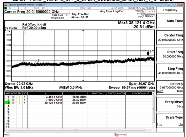
Band77-Part27_100MHz_DFT_s_OFDM_SCS30kHz_BPSK_RB1_1_CH633334
