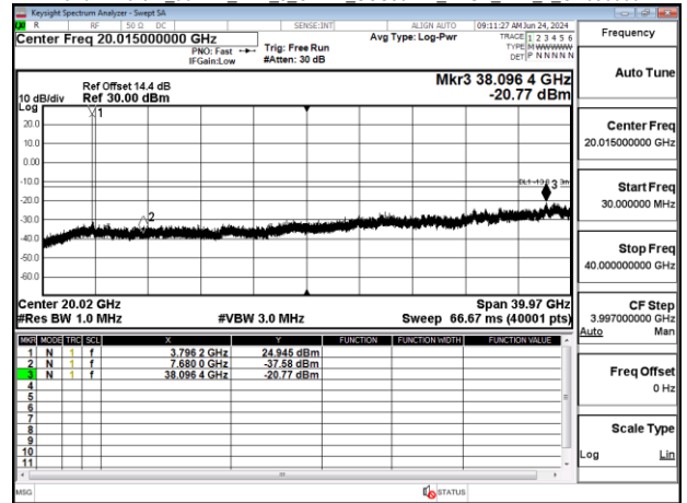
Band77-Part27_90MHz_DFT_s_OFDM_SCS30kHz_BPSK_RB1_1_CH662332
