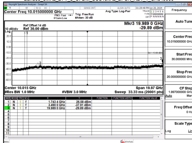
Band66_5MHz_DFT_s_OFDM_SCS15kHz_BPSK_RB1_1_CH355500
