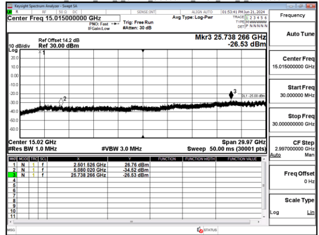
Band41_80MHz_DFT_s_OFDM_SCS30kHz_BPSK_RB1_1_CH518598
