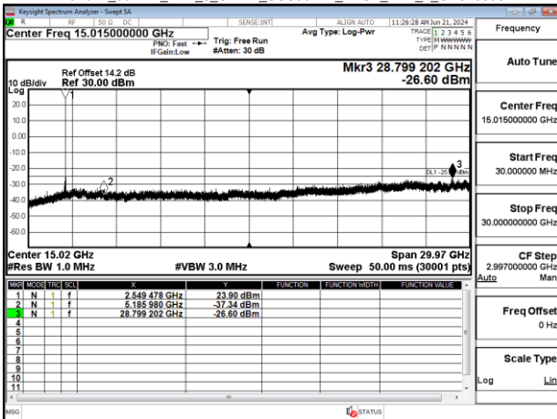
Band41_90MHz_DFT_s_OFDM_SCS30kHz_BPSK_RB1_1_CH518598
