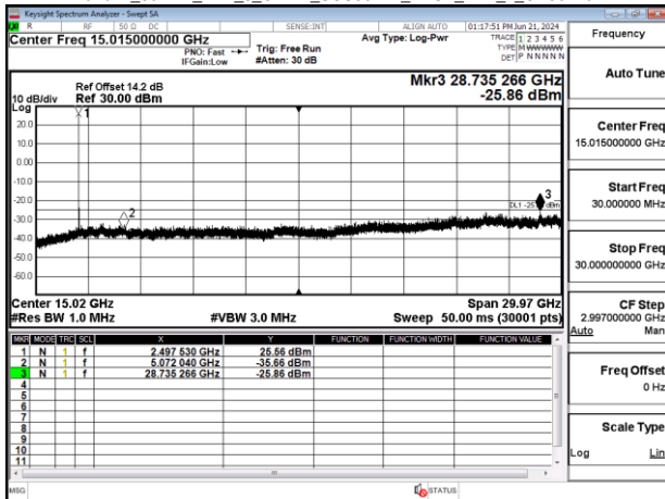
Band41_80MHz_DFT_s_OFDM_SCS30kHz_BPSK_RB1_1_CH507204
