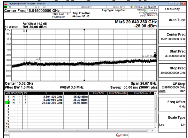
Band41_100MHz_DFT_s_OFDM_SCS30kHz_BPSK_RB1_1_CH509202
