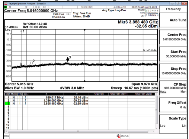
Band71_15MHz_DFT_s_OFDM_SCS15kHz_BPSK_RB1_1_CH134100
