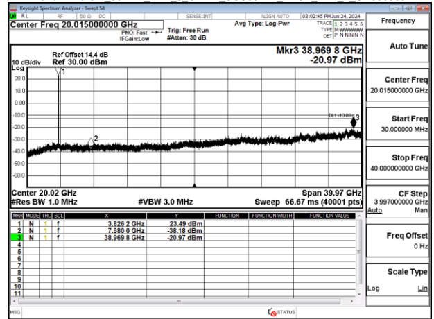
Band77-Part27_30MHz_DFT_s_OFDM_SCS30kHz_BPSK_RB1_1_CH664332
