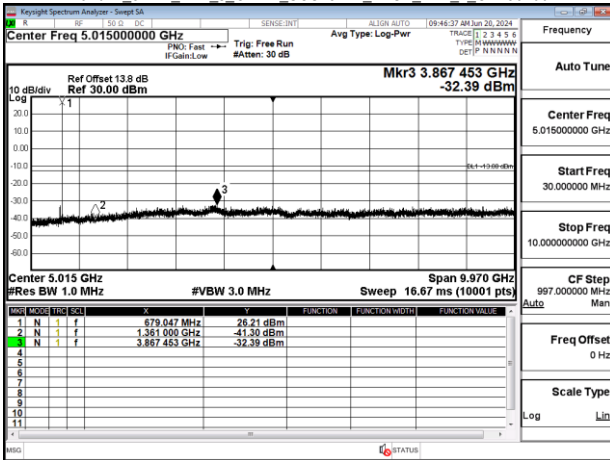
Band71_5MHz_DFT_s_OFDM_SCS15kHz_BPSK_RB1_1_CH139100
