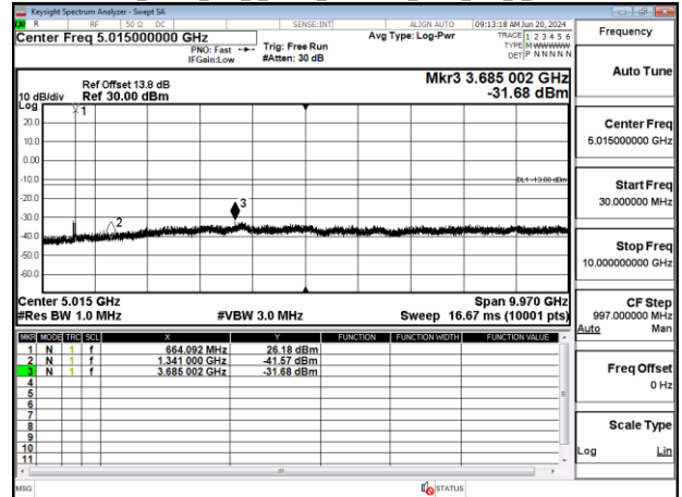
Band71_15MHz_DFT_s_OFDM_SCS15kHz_BPSK_RB1_1_CH134100
