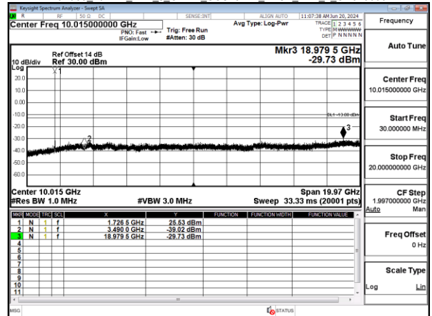
Band66 40MHz DFT s_OFDM_SCS15kHz BPSK_RB1_1_CH352000
