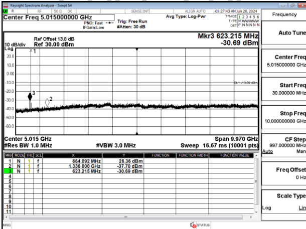
Band71_10MHz_DFT_s_OFDM_SCS15kHz_BPSK_RB1_1_CH133600
