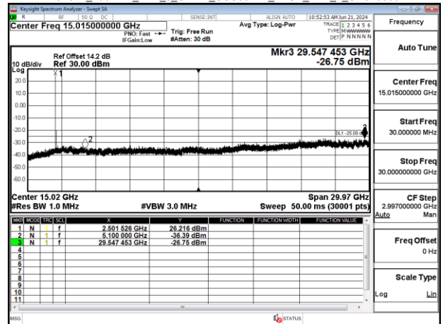
Band41_100MHz_DFT_s_OFDM_SCS30kHz_BPSK_RB1_1_CH510000
