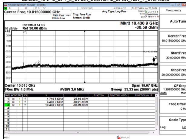
Band66_10MHz_DFT_s_OFDM_SCS15kHz_BPSK_RB1_1_CH343000
