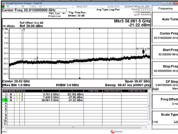
Band77-Part27_30MHz_DFT_s_OFDM_SCS30kHz_BPSK_RB1_1_CH647668
