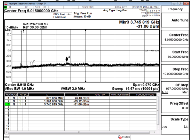
Band71_10MHz_DFT_s_OFDM_SCS15kHz_BPSK_RB1_1_CH138600
