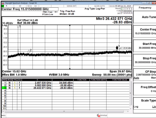
Band41_90MHz_DFT_s_OFDM_SCS30kHz_BPSK_RB1_1_CH509004
