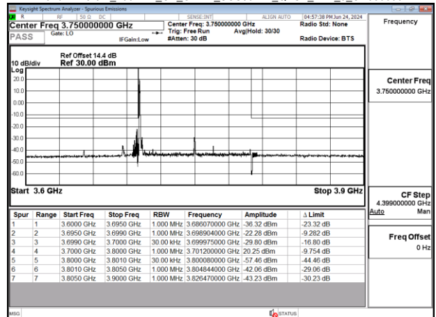
Band77-Part27_100MHz_CP_OFDM_SCS30kHz_QPSK_RB1_0_CH650000
