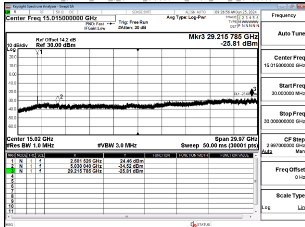
Band41_30MHz_DFT_s_OFDM_SCS30kHz_BPSK_RB1_1_CH503004
