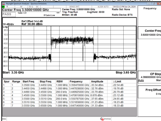
Band77-Part27_100MHz_CP_OFDM_SCS30kHz_QPSK_RB273_0_CH650000
