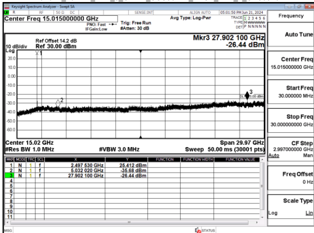
Band41_40MHz_DFT_s_OFDM_SCS30kHz_BPSK_RB1_1_CH503202
