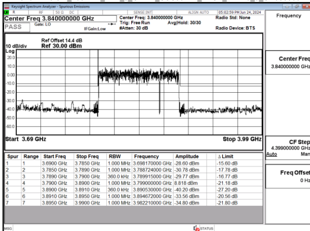
Band77-Part27_100MHz_DFT_s_OFDM_SCS30kHz_BPSK_RB270_0_CH656000
