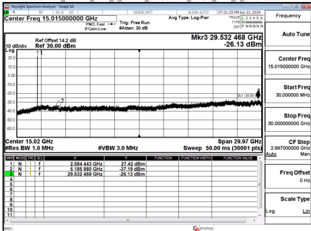
Band41_20MHz_DFT_s_OFDM_SCS30kHz_BPSK_RB1_1_CH518598
