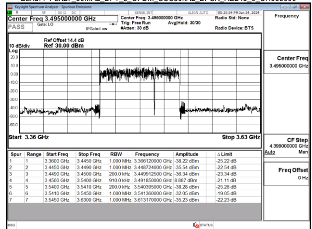
Band77-Part27_90MHz_DFT_s_OFDM_SCS30kHz_BPSK_RB243_0_CH633334
