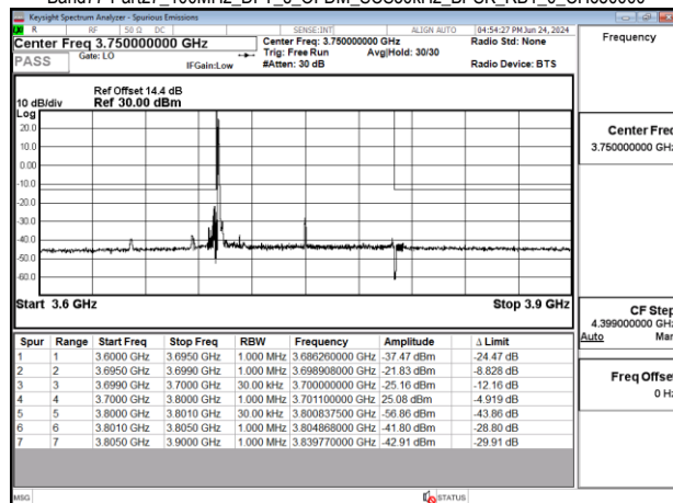
Band77-Part27_100MHz_DFT_s_OFDM_SCS30kHz_BPSK_RB1_0_CH650000
