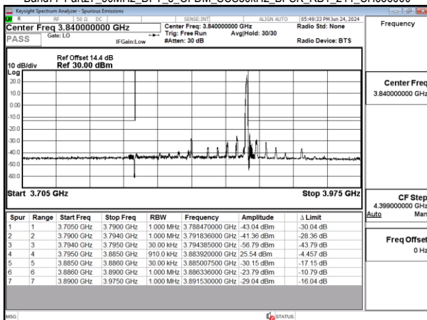
Band77-Part27_90MHz_DFT_s_OFDM_SCS30kHz_BPSK_RB1_244_CH656000
