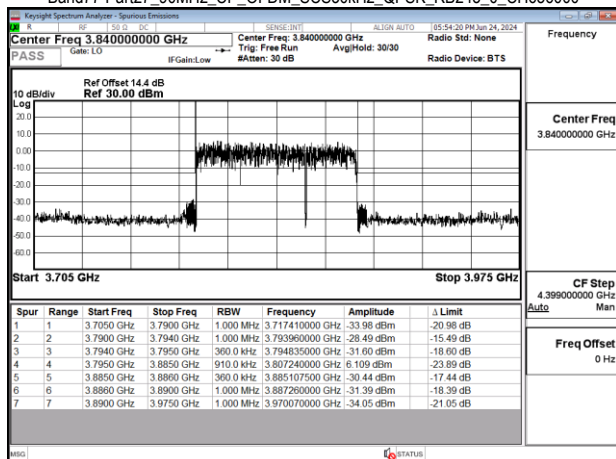
Band77-Part27_90MHz_CP_OFDM_SCS30kHz_QPSK_RB245_0_CH656000
