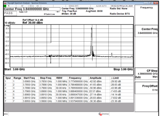
Band77-Part27_100MHz_DFT_s_OFDM_SCS30kHz_BPSK_RB1_272_CH662000
