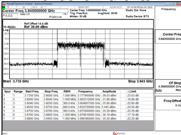
Band77-Part27_70MHz_CP_OFDM_SCS30kHz_QPSK_RB189_0_CH656000
