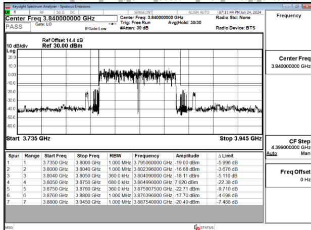
Band77-Part27_70MHz_DFT_s_OFDM_SCS30kHz_BPSK_RB180_0_CH656000
