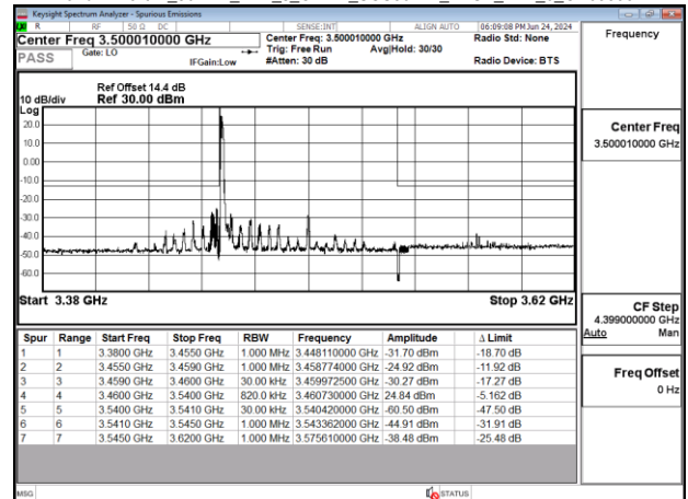
Band77-Part27_80MHz_DFT_s_OFDM_SCS30kHz_BPSK_RB1_0_CH633334
