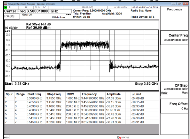
Band77-Part27_80MHz_DFT_s_OFDM_SCS30kHz_BPSK_RB216_0_CH633334
