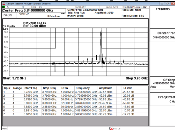
Band77-Part27_80MHz_DFT_s_OFDM_SCS30kHz_BPSK_RB1_216_CH656000
