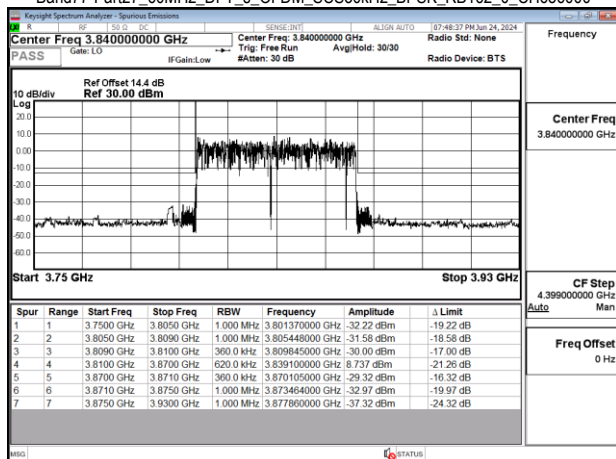
Band77-Part27_60MHz_DFT_s_OFDM_SCS30kHz_BPSK_RB162_0_CH656000
