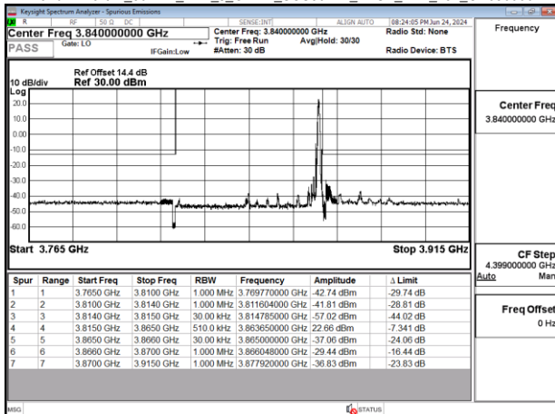
Band77-Part27_50MHz_DFT_s_OFDM_SCS30kHz_BPSK_RB1_132_CH656000
