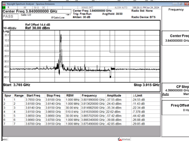
Band77-Part27_50MHz_CP_OFDM_SCS30kHz_QPSK_RB1_0_CH656000
