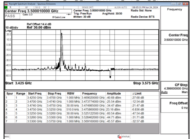
Band77-Part27_50MHz_DFT_s_OFDM_SCS30kHz_BPSK_RB1_0_CH633334
