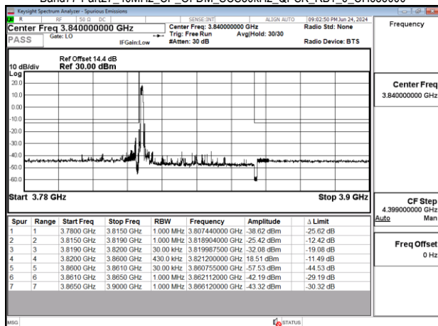
Band77-Part27_40MHz_CP_OFDM_SCS30kHz_QPSK_RB1_0_CH656000
