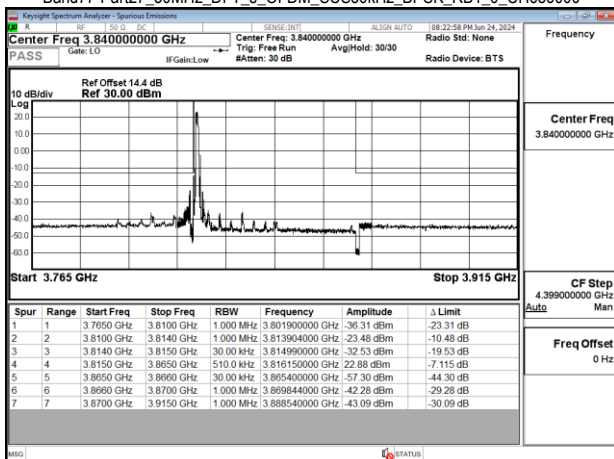
Band77-Part27_50MHz_DFT_s_OFDM_SCS30kHz_BPSK_RB1_0_CH656000
