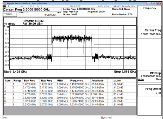
Band77-Part27_50MHz_DFT_s_OFDM_SCS30kHz_BPSK_RB128_0_CH633334
