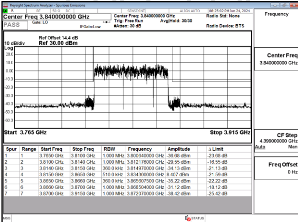
Band77-Part27_50MHz_DFT_s_OFDM_SCS30kHz_BPSK_RB128_0_CH656000
