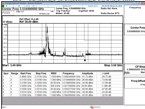
Band77-Part27_30MHz_CP_OFDM_SCS30kHz_QPSK_RB1_0_CH647668
