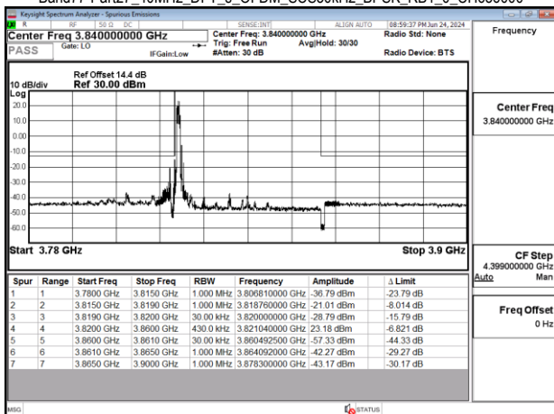
Band77-Part27_40MHz_DFT_s_OFDM_SCS30kHz_BPSK_RB1_0_CH656000
