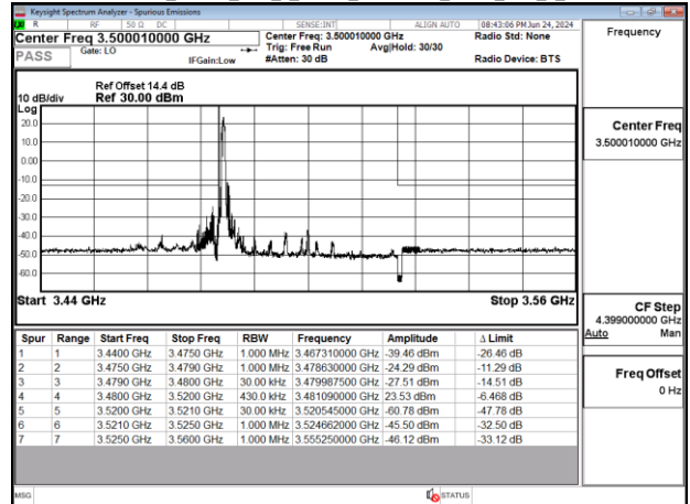
Band77-Part27_40MHz_DFT_s_OFDM_SCS30kHz_BPSK_RB1_0_CH633334
