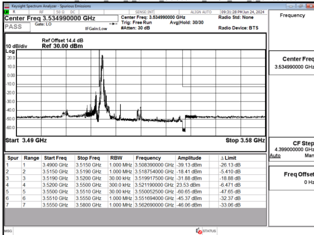
Band77-Part27_30MHz_DFT_s_OFDM_SCS30kHz_BPSK_RB1_0_CH647668
