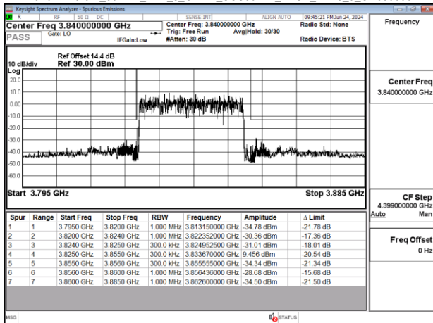
Band77-Part27_30MHz_DFT_s_OFDM_SCS30kHz_BPSK_RB75_0_CH656000
