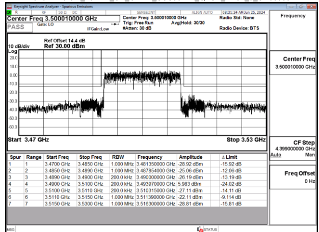
Band77-Part27_20MHz_CP_OFDM_SCS30kHz_QPSK_RB51_0_CH633334
