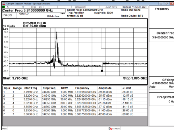
Band77-Part27_30MHz_DFT_s_OFDM_SCS30kHz_BPSK_RB1_0_CH656000
