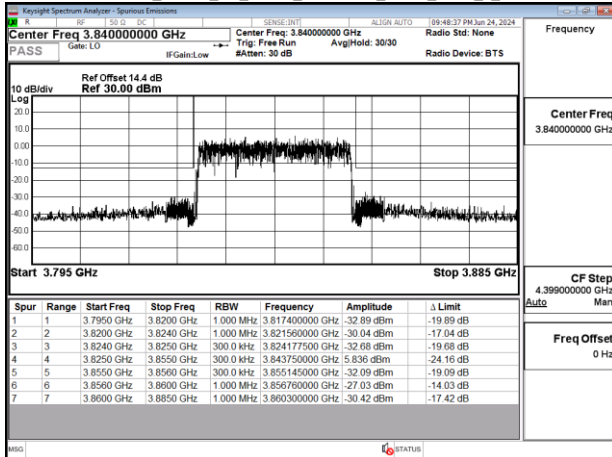
Band77-Part27_30MHz_CP_OFDM_SCS30kHz_QPSK_RB78_0_CH656000
