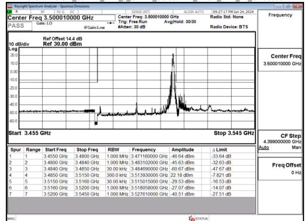
Band77-Part27_30MHz_DFT_s_OFDM_SCS30kHz_BPSK_RB1_77_CH633334
