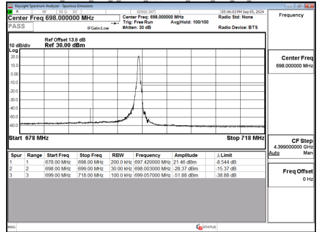
Band71 20MHz DFT_s_OFDM_SCS15kHz_BPSK_RB100_0_CH134600
