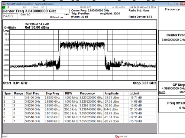
Band77-Part27_20MHz_DFT_s_OFDM_SCS30kHz_BPSK_RB50_0_CH656000
