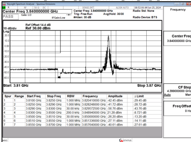
Band77-Part27_20MHz_DFT_s_OFDM_SCS30kHz_BPSK_RB1_50_CH656000
