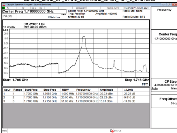
Band66_5MHz_CP_OFDM_SCS15kHz_QPSK_RB1_0_CH342500
