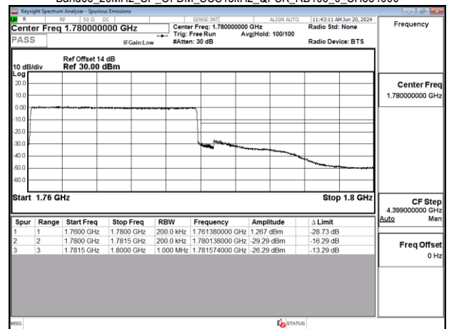
Band66_20MHz_CP_OFDM_SCS15kHz_QPSK_RB106_0_CH354000
