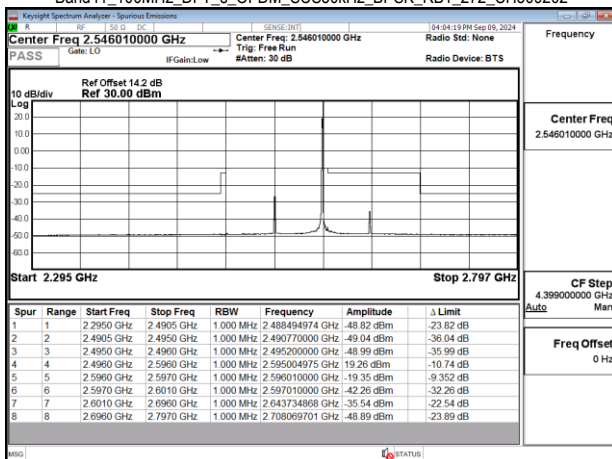
Band41_100MHz_DFT_s_OFDM_SCS30kHz_BPSK_RB1_272_CH509202
