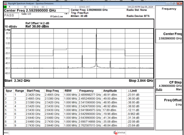
Band41_100MHz_CP_OFDM_SCS30kHz_QPSK_RB1_272_CH528000
