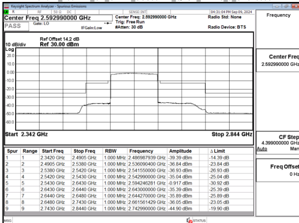
Band41_100MHz_CP_OFDM_SCS30kHz_QPSK_RB273_0_CH518598
