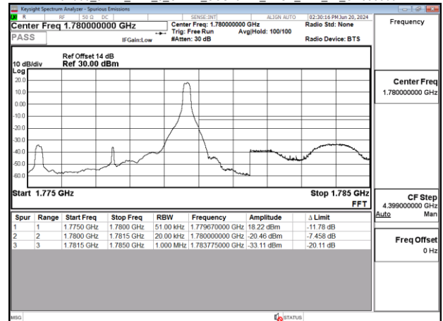
Band66_5MHz_DFT_s_OFDM_SCS15kHz_BPSK_RB1_24_CH355500
