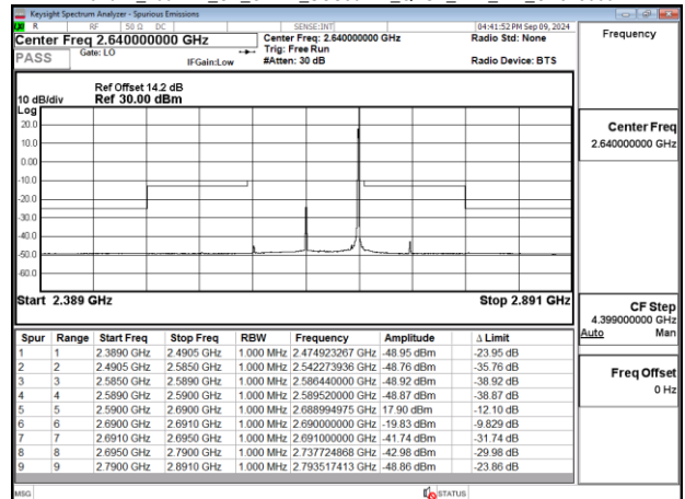
Band41_100MHz_CP_OFDM_SCS30kHz_QPSK_RB1_272_CH528000
