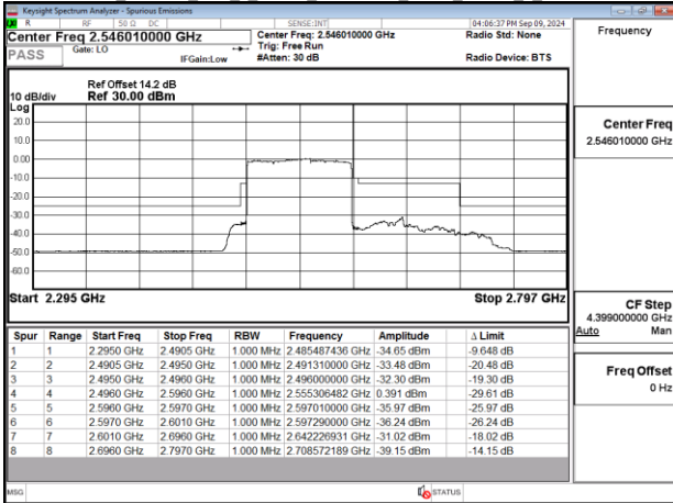
Band41_100MHz_DFT_s_OFDM_SCS30kHz_BPSK_RB270_0_CH510000
