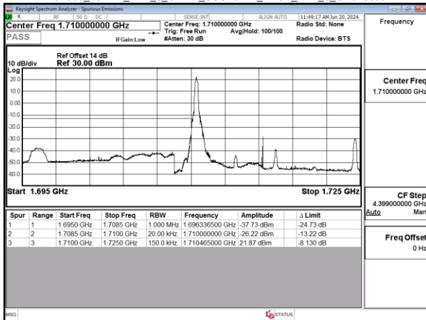
Band66_15MHz_DFT_s_OFDM_SCS15kHz_BPSK_RB1_0_CH343500
