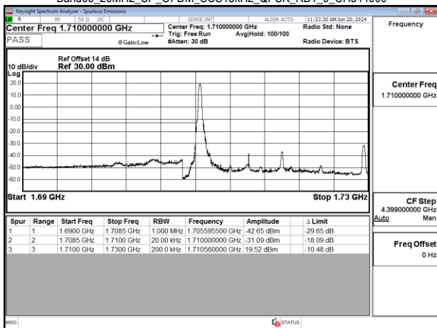
Band66_20MHz_CP_OFDM_SCS15kHz_QPSK_RB1_0_CH344000
