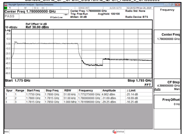
Band66_5MHz_CP_OFDM_SCS15kHz_QPSK_RB25_0_CH355500
