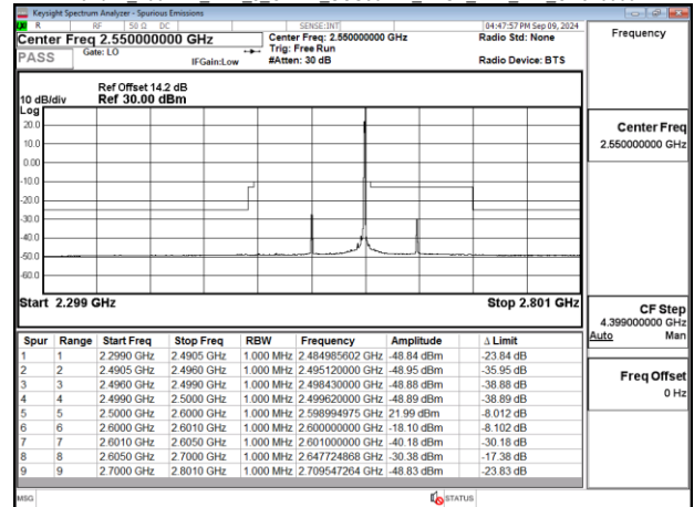
Band41_100MHz_DFT_s_OFDM_SCS30kHz_BPSK_RB1_272_CH518598
