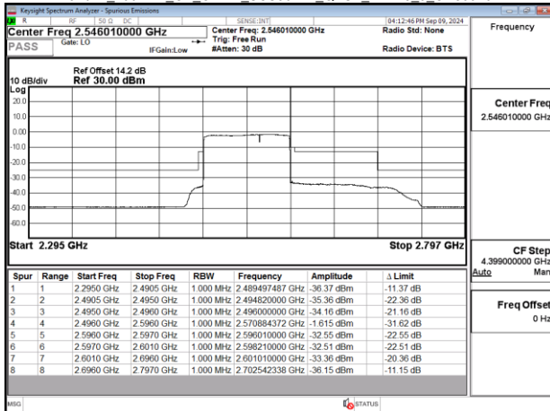
Band41_100MHz_CP_OFDM_SCS30kHz_QPSK_RB273_0_CH510000
