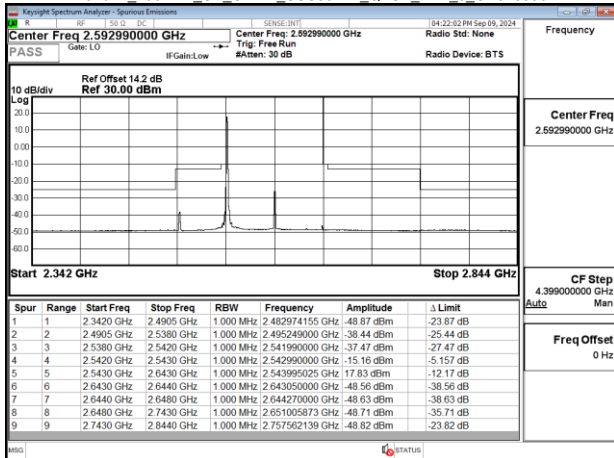
Band41_100MHz_CP_OFDM_SCS30kHz_QPSK_RB1_0_CH528000
