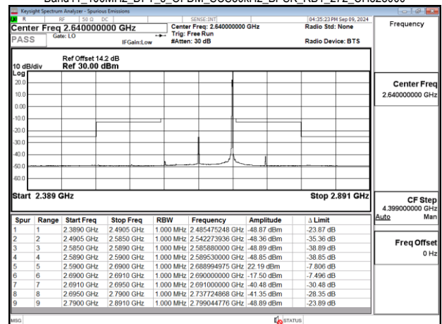
Band41_100MHz_DFT_s_OFDM_SCS30kHz_BPSK_RB1_272_CH528000
