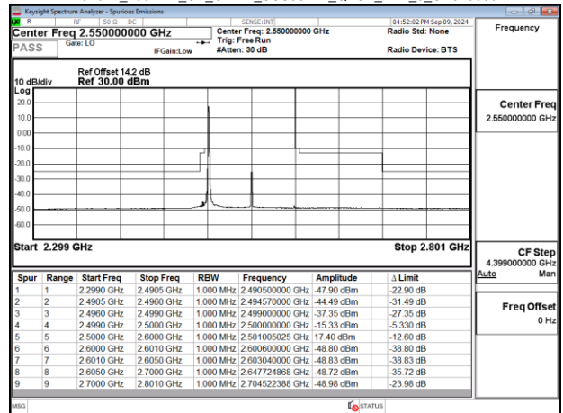
Band41_100MHz_CP_OFDM_SCS30kHz_QPSK_RB1_0_CH510000
