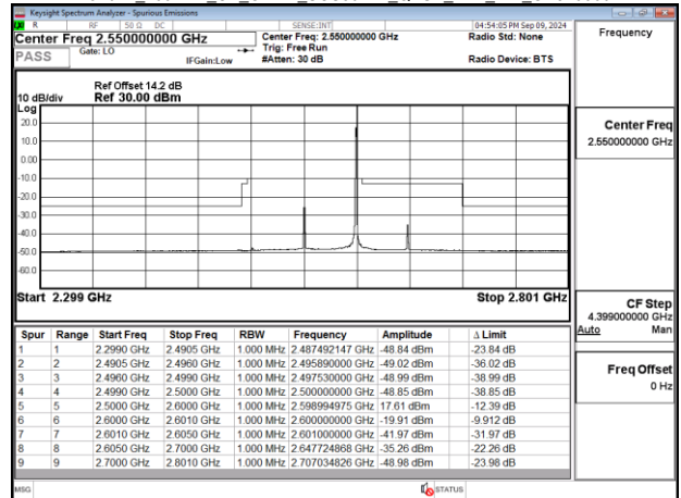
Band41_100MHz_CP_OFDM_SCS30kHz_QPSK_RB1_272_CH518598
