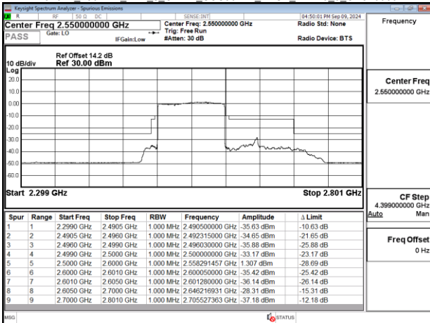
Band41_100MHz_DFT_s_OFDM_SCS30kHz_BPSK_RB270_0_CH518598
