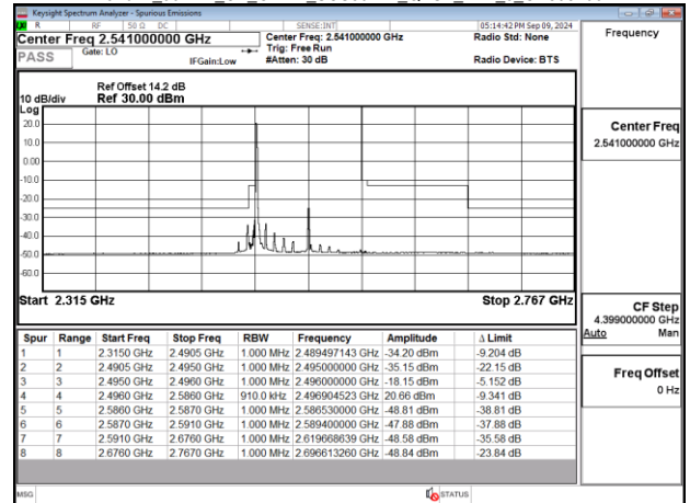
Band41_90MHz_CP_OFDM_SCS30kHz_QPSK_RB1_0_CH509004
