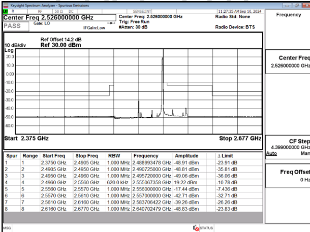
Band41_60MHz_DFT_s_OFDM_SCS30kHz_BPSK_RB1_161_CH505200
