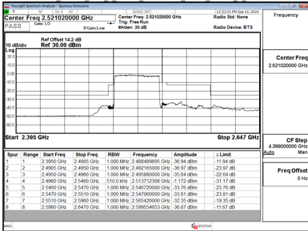
Band41_50MHz_DFT_s_OFDM_SCS30kHz_BPSK_RB128_0_CH505002
