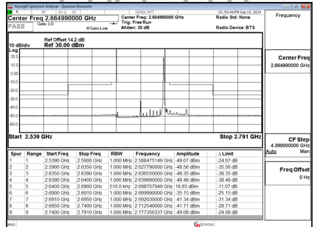
Band41_50MHz_DFT_s_OFDM_SCS30kHz_BPSK_RB1_132_CH532998
