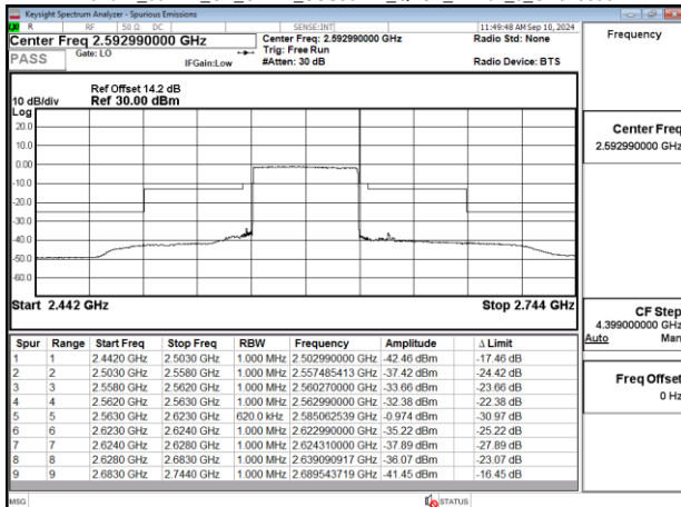
Band41_60MHz_CP_OFDM_SCS30kHz_QPSK_RB162_0_CH518598
