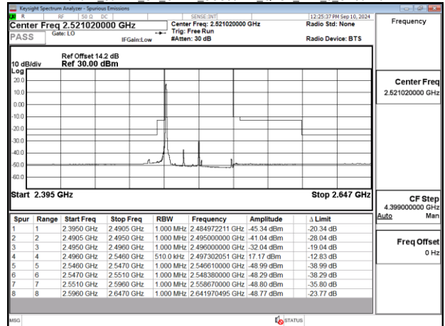
Band41_50MHz_CP_OFDM_SCS30kHz_QPSK_RB1_0_CH505002
