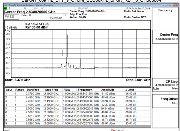
Band41 60MHz DFT_s OFDM_SCS30kHz BPSK RB1 0_CH506004
