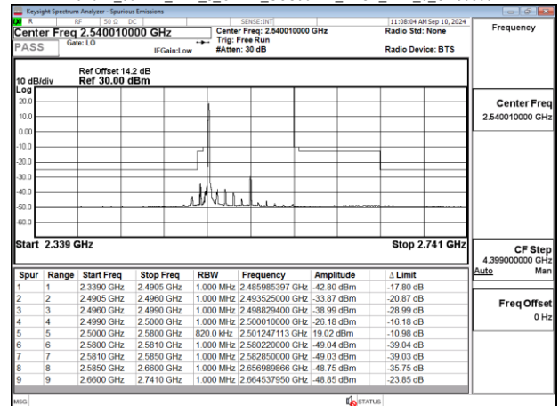
Band41_80MHz_DFT_s_OFDM_SCS30kHz_BPSK_RB1_0_CH508002
