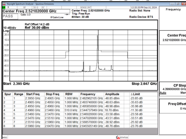
Band41_50MHz_DFT_s_OFDM_SCS30kHz_BPSK_RB1_132_CH504204
