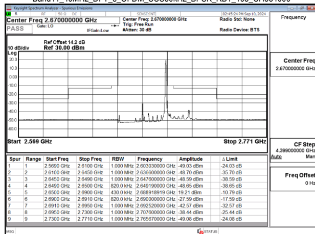
Band41 40MHz DFT s OFDM_SCS30kHz BPSK RB1_105_CH534000
