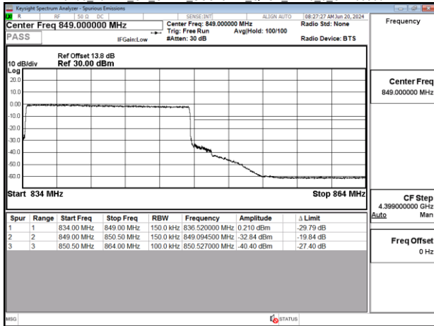
Band5_20MHz_DFT_s_OFDM_SCS15kHz_BPSK_RB1_0_CH166800
