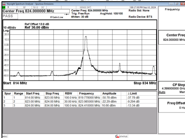
Band5_10MHz_CP_OFDM_SCS15kHz_QPSK_RB1_0_CH165800
