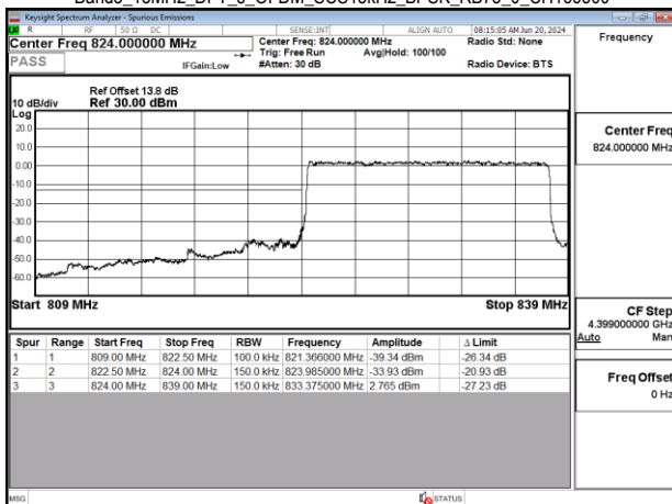
Band5_15MHz_DFT_s_OFDM_SCS15kHz_BPSK_RB75_0_CH166300
