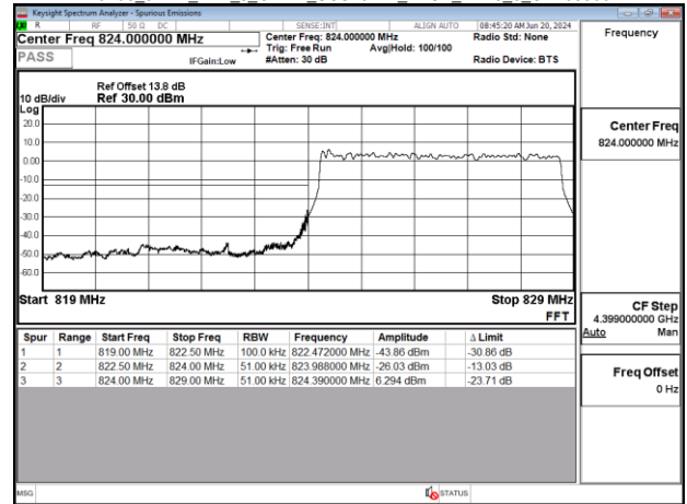
Band5 5MHz DFT_s_OFDM_SCS15kHz BPSK RB25_0 CH169300
