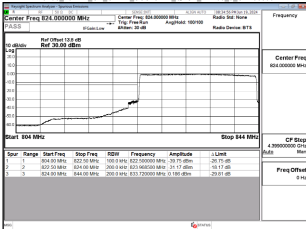
Band5_20MHz_CP_OFDM_SCS15kHz_QPSK_RB106_0_CH166800
