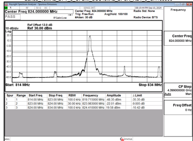
Band5 10MHz DFT_s_OFDM_SCS15kHz_BPSK_RB1_51_CH168800
