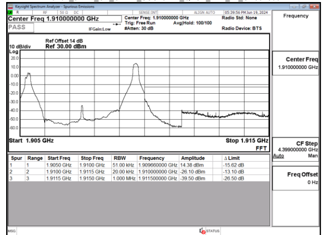
Band2_5MHz_CP_OFDM_SCS15kHz_QPSK_RB1_24_CH381500
