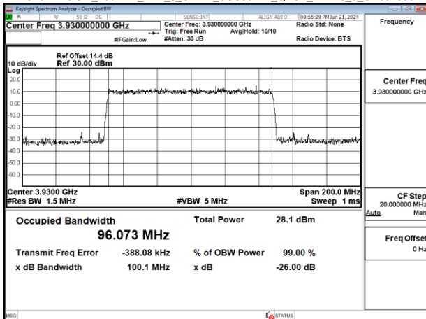
Band77-Part27_100MHz_DFT_s_OFDM_SCS30kHz_QPSK_RB270_0_CH662000
