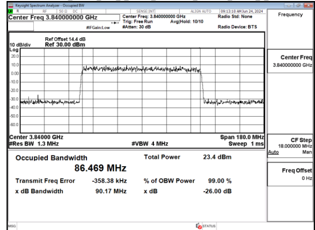
Band77-Part27 90MHz DFT s_OFDM_SCS30kHz 256QAM_RB243_0_CH656000
