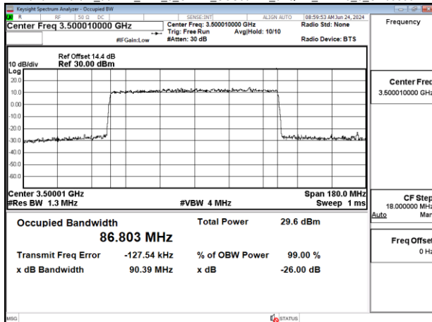
Band77-Part27_90MHz_DFT_s_OFDM_SCS30kHz_64QAM_RB243_0_CH633334
