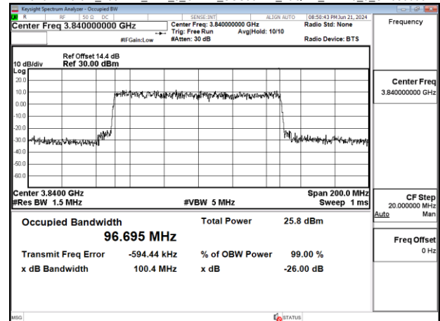
Band77-Part27_100MHz_DFT_s_OFDM_SCS30kHz_16QAM_RB270_0_CH656000
