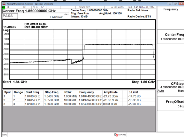
Band2_10MHz_CP_OFDM_SCS15kHz_QPSK_RB52_0_CH371000
