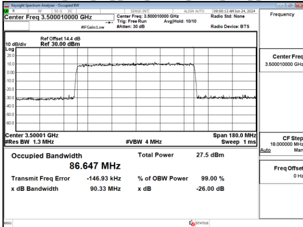
Band77-Part27 90MHz DFT s_OFDM_SCS30kHz 256QAM_RB243_0_CH633334
