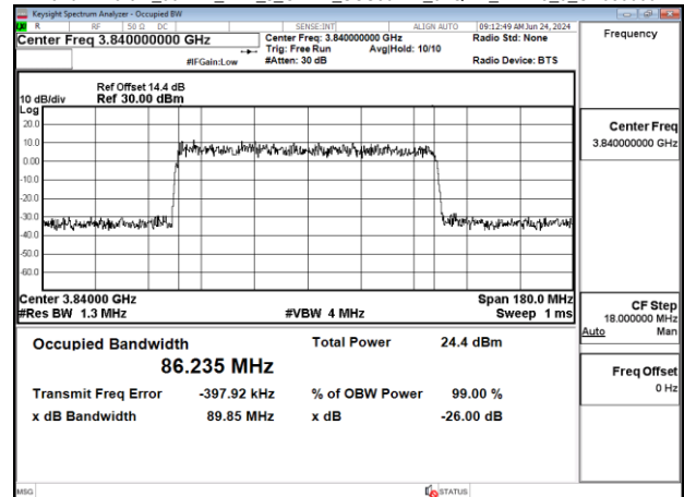
Band77-Part27_90MHz_DFT_s_OFDM_SCS30kHz_64QAM_RB243_0_CH656000
