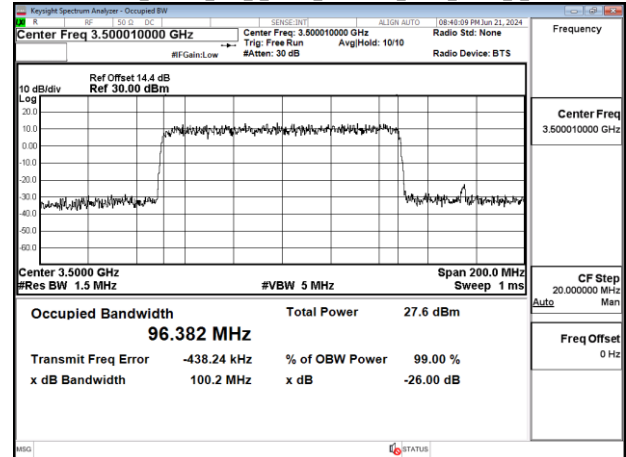
Band77-Part27_100MHz_DFT_s_OFDM_SCS30kHz_QPSK_RB270_0_CH633334
