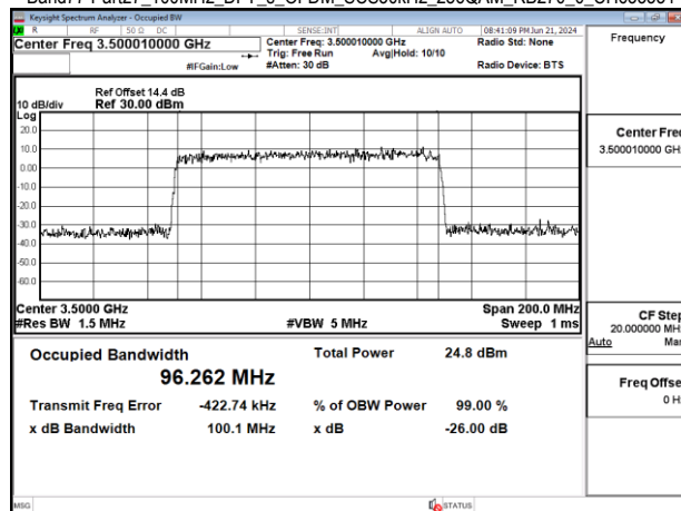
Band77-Part27_100MHz_DFT_s_OFDM_SCS30kHz_256QAM_RB270_0_CH633334
