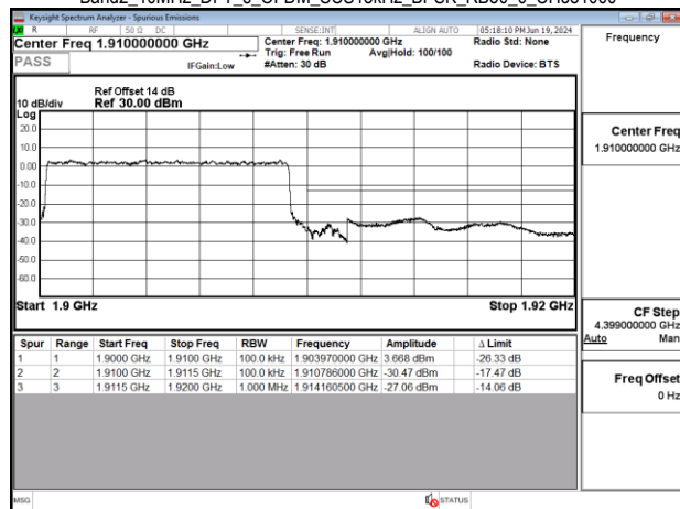
Band2_10MHz_DFT_s_OFDM_SCS15kHz_BPSK_RB50_0_CH381000
