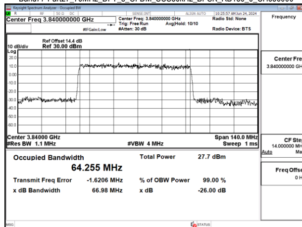
Band77-Part27_70MHz_DFT_s_OFDM_SCS30kHz_BPSK_RB180_0_CH656000
