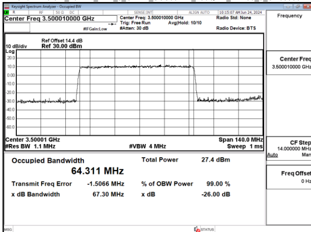
Band77-Part27 70MHz DFT s OFDM_SCS30kHz 256QAM_RB180_0_CH633334
