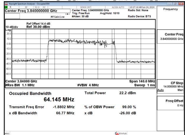
Band77-Part27 70MHz DFT s OFDM_SCS30kHz 256QAM_RB180_0_CH656000
