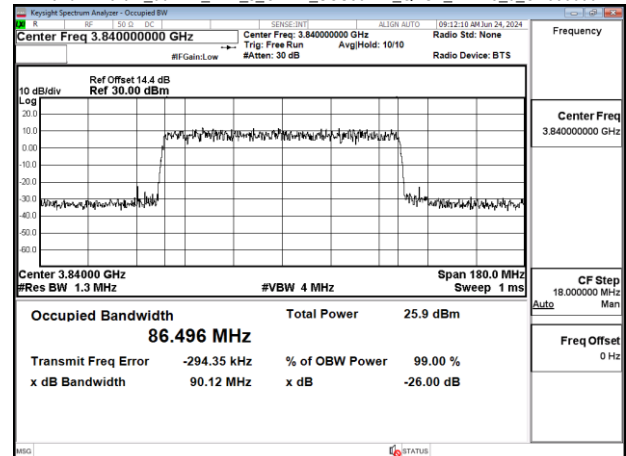
Band77-Part27_90MHz_DFT_s_OFDM_SCS30kHz_QPSK_RB243_0_CH656000
