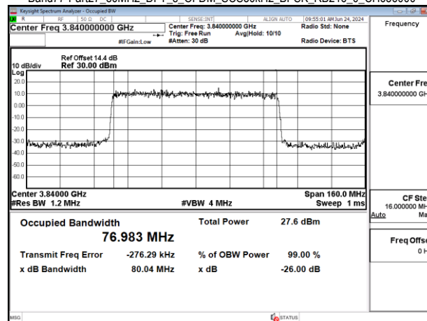
Band77-Part27_80MHz_DFT_s_OFDM_SCS30kHz_BPSK_RB216_0_CH656000
