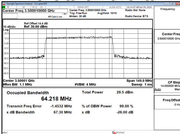
Band77-Part27_70MHz_DFT_s_OFDM_SCS30kHz_64QAM_RB180_0_CH633334
