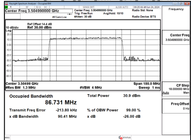
Band77-Part27_90MHz_DFT_s_OFDM_SCS30kHz_QPSK_RB243_0_CH649668
