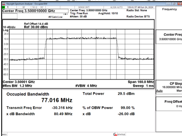
Band77-Part27_80MHz_DFT_s_OFDM_SCS30kHz_64QAM_RB216_0_CH633334
