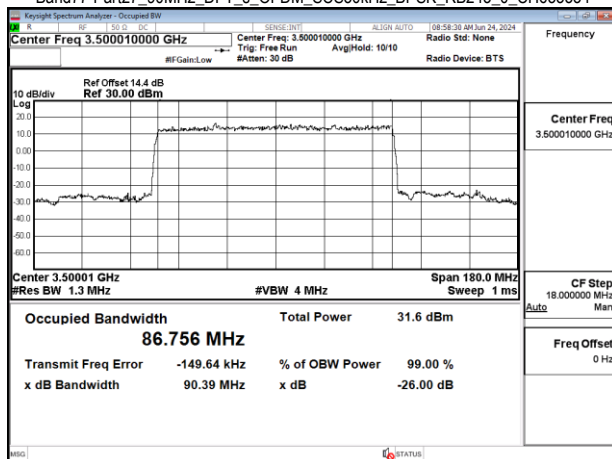
Band77-Part27_90MHz_DFT_s_OFDM_SCS30kHz_BPSK_RB243_0_CH633334
