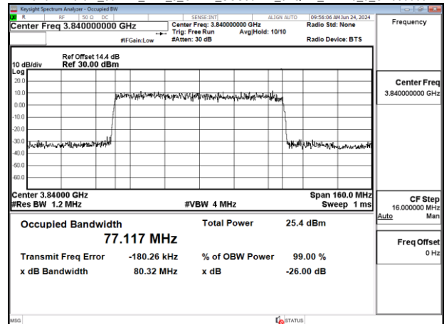
Band77-Part27_80MHz_DFT_s_OFDM_SCS30kHz_64QAM_RB216_0_CH656000
