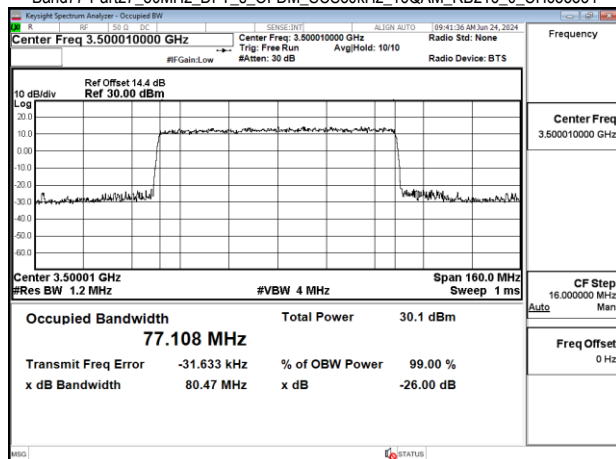
Band77-Part27_80MHz_DFT_s_OFDM_SCS30kHz_16QAM_RB216_0_CH633334
