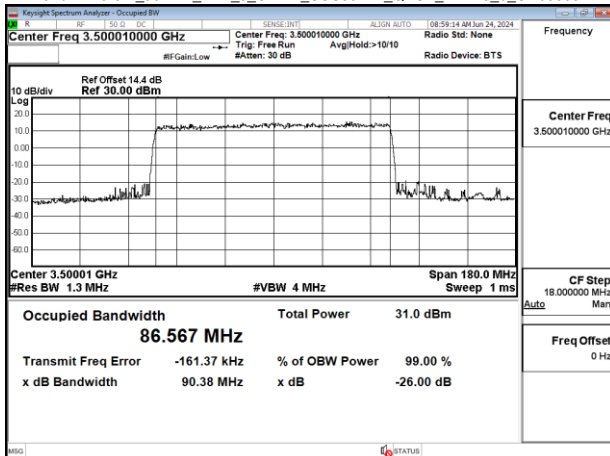
Band77-Part27_90MHz_DFT_s_OFDM_SCS30kHz_QPSK_RB243_0_CH633334
