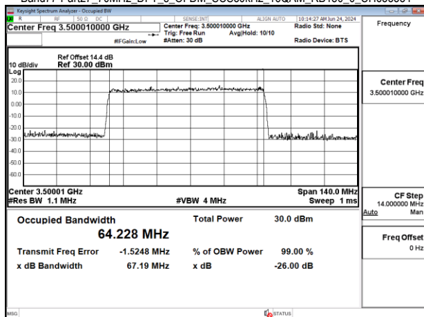
Band77-Part27_70MHz_DFT_s_OFDM_SCS30kHz_16QAM_RB180_0_CH633334
