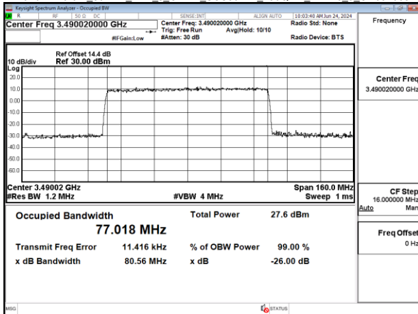
Band77-Part27 80MHz DFT s_OFDM_SCS30kHz 256QAM_RB216_0_CH633334
