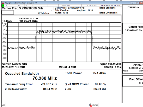
Band77-Part27_80MHz_DFT_s_OFDM_SCS30kHz_64QAM_RB216_0_CH662668
