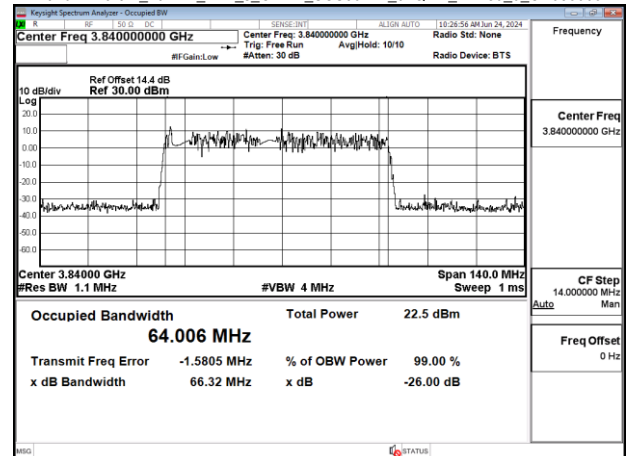
Band77-Part27_70MHz_DFT_s_OFDM_SCS30kHz_64QAM_RB180_0_CH656000
