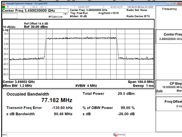
Band77-Part27_80MHz_DFT_s_OFDM_SCS30kHz_64QAM_RB216_0_CH633334
