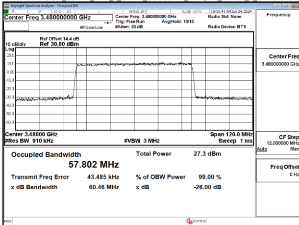
Band77-Part27 60MHz DFT s_OFDM_SCS30kHz 256QAM_RB162_0_CH63334
