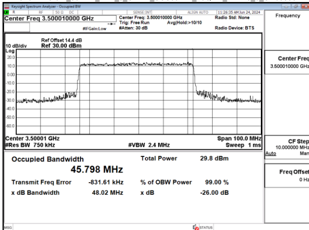
Band77-Part27_50MHz_DFT_s_OFDM_SCS30kHz_16QAM_RB128_0_CH633334
