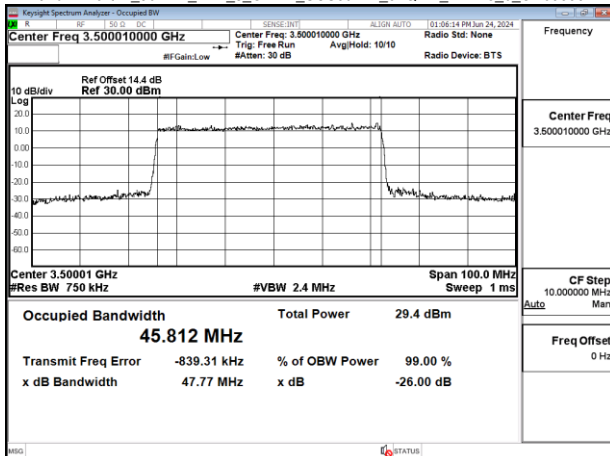
Band77-Part27_50MHz_DFT_s_OFDM_SCS30kHz_64QAM_RB128_0_CH633334
