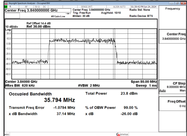
Band77-Part27_40MHz_DFT_s_OFDM_SCS30kHz_64QAM_RB100_0_CH656000
