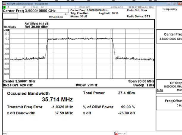
Band77-Part27 40MHz DFT s_OFDM_SCS30kHz 256QAM_RB100_0_CH633334
