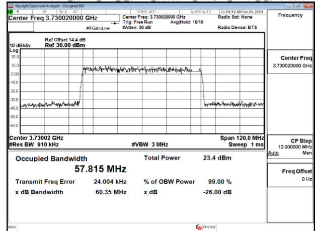
Band77-Part27 60MHz DFT s_OFDM_SCS30kHz 256QAM_RB162_0_CH65600
