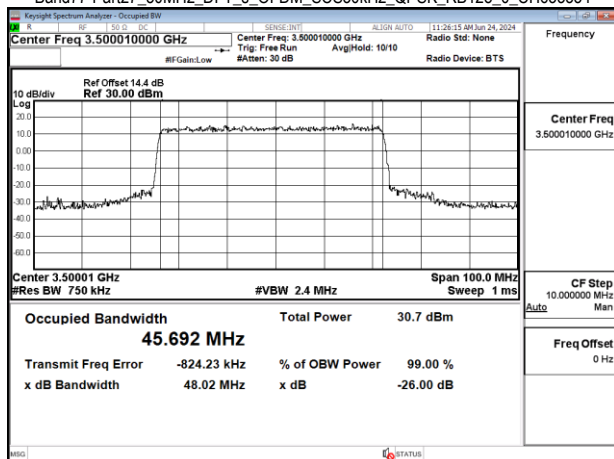
Band77-Part27_50MHz_DFT_s_OFDM_SCS30kHz_QPSK_RB128_0_CH633334
