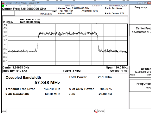
Band77-Part27 60MHz DFT s_OFDM_SCS30kHz 256QAM_RB162_0_CH63200
