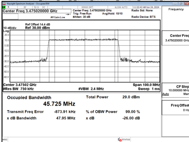
Band77-Part27 50MHz DFT s_OFDM_SCS30kHz 256QAM_RB128_0_CH633334
