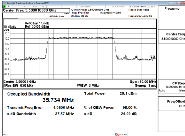
Band77-Part27_40MHz_DFT_s_OFDM_SCS30kHz_64QAM_RB100_0_CH633334
