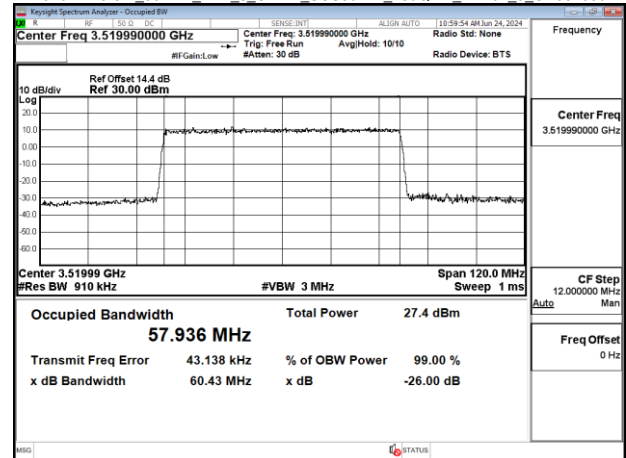
Band77-Part27 60MHz DFT s_OFDM_SCS30kHz 256QAM_RB162_0_CH64868
