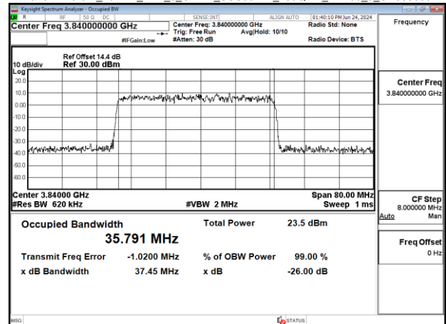
Band77-Part27 40MHz DFT s_OFDM_SCS30kHz 256QAM_RB100_0_CH656000
