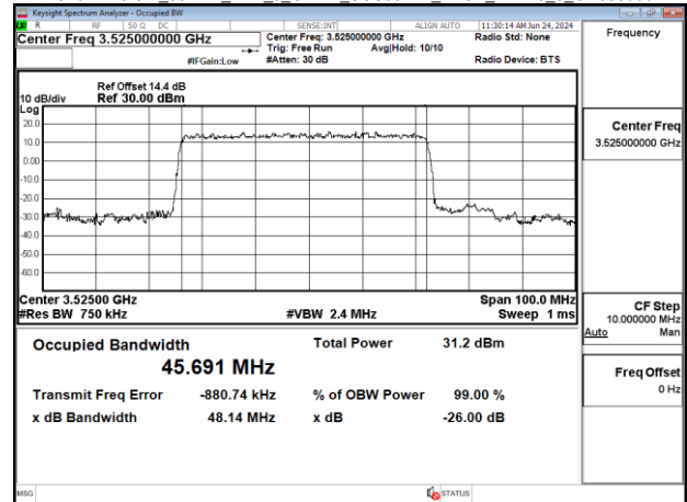
Band77-Part27_50MHz_DFT_s_OFDM_SCS30kHz_BPSK_RB128_0_CH648334
