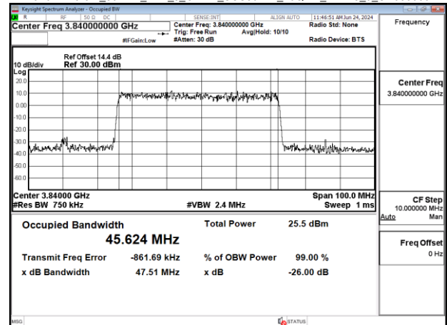
Band77-Part27_50MHz_DFT_s_OFDM_SCS30kHz_16QAM_RB128_0_CH656000
