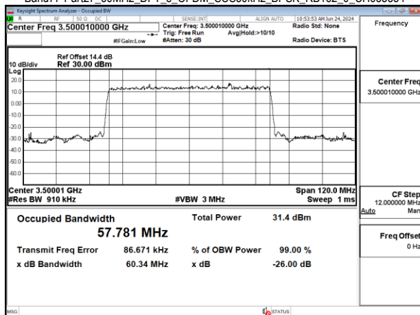
Band77-Part27_60MHz_DFT_s_OFDM_SCS30kHz_BPSK_RB162_0_CH633334
