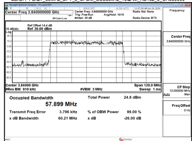
Band77-Part27_60MHz_DFT_s_OFDM_SCS30kHz_16QAM_RB162_0_CH656000
