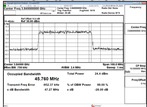
Band77-Part27_50MHz_DFT_s_OFDM_SCS30kHz_64QAM_RB128_0_CH656000
