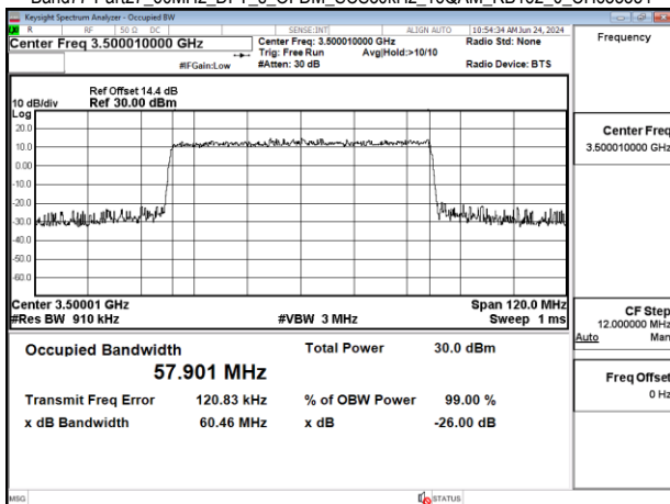
Band77-Part27_60MHz_DFT_s_OFDM_SCS30kHz_16QAM_RB162_0_CH633334
