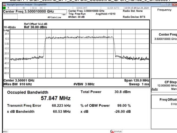
Band77-Part27_60MHz_DFT_s_OFDM_SCS30kHz_QPSK_RB162_0_CH633334
