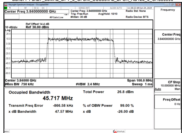
Band77-Part27_50MHz_DFT_s_OFDM_SCS30kHz_BPSK_RB128_0_CH656000
