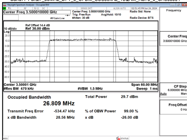
Band77-Part27_30MHz_DFT_s_OFDM_SCS30kHz_16QAM_RB75_0_CH633334
