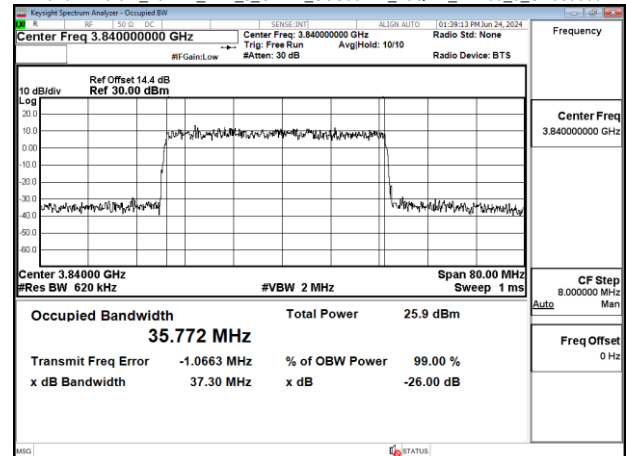
Band77-Part27_40MHz_DFT_s_OFDM_SCS30kHz_16QAM_RB100_0_CH656000
