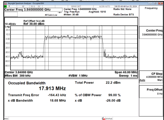
Band77-Part27_20MHz_DFT_s_OFDM_SCS30kHz_256QAM_RB50_0_CH656000
