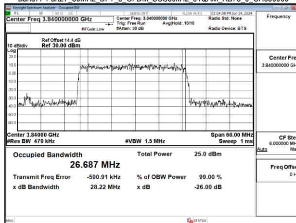
Band77-Part27_30MHz_DFT_s_OFDM_SCS30kHz_64QAM_RB75_0_CH656000
