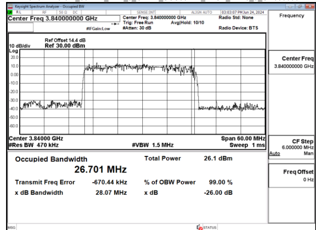
Band77-Part27_30MHz_DFT_s_OFDM_SCS30kHz_BPSK_RB75_0_CH656000
