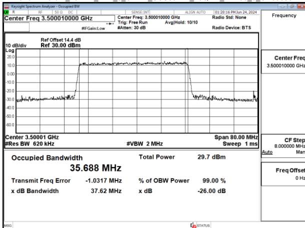
Band77-Part27_40MHz_DFT_s_OFDM_SCS30kHz_16QAM_RB100_0_CH633334
