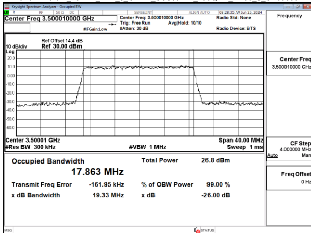
Band77-Part27_20MHz_DFT_s_OFDM_SCS30kHz_256QAM_RB50_0_CH633334
