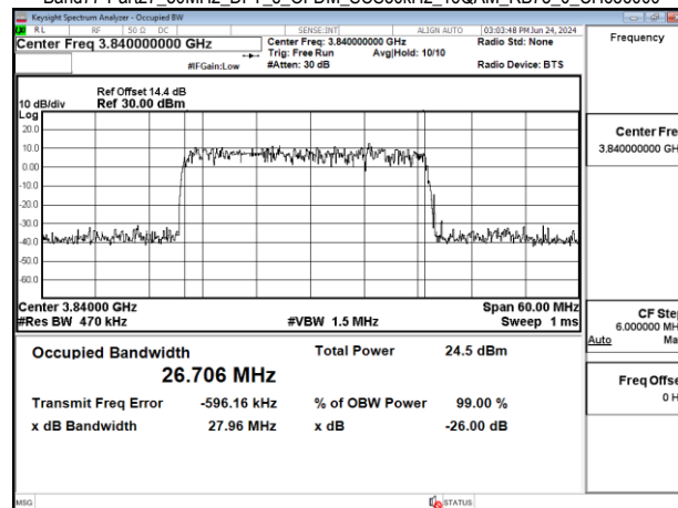
Band77-Part27_30MHz_DFT_s_OFDM_SCS30kHz_16QAM_RB75_0_CH656000
