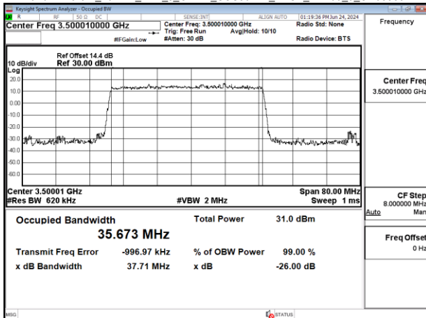
Band77-Part27 40MHz_DFT_s_OFDM_SCS30kHz_BPSK_RB100_0_CH633334
