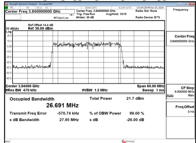
Band77-Part27_30MHz_DFT_s_OFDM_SCS30kHz_256QAM_RB75_0_CH656000
