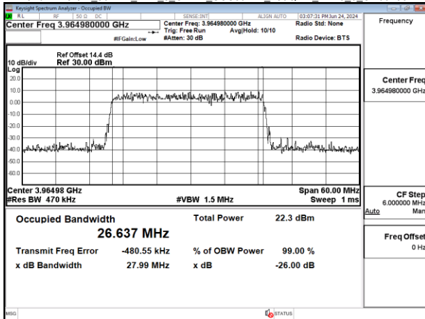
Band77-Part27 40MHz_DFT_s_OFDM_SCS30kHz_BPSK_RB100_0_CH631334
