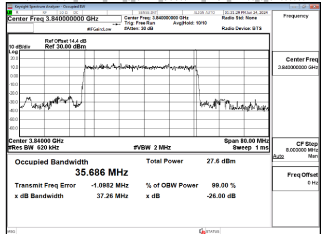
Band77-Part27 40MHz_DFT_s_OFDM_SCS30kHz_BPSK_RB100_0_CH656000
