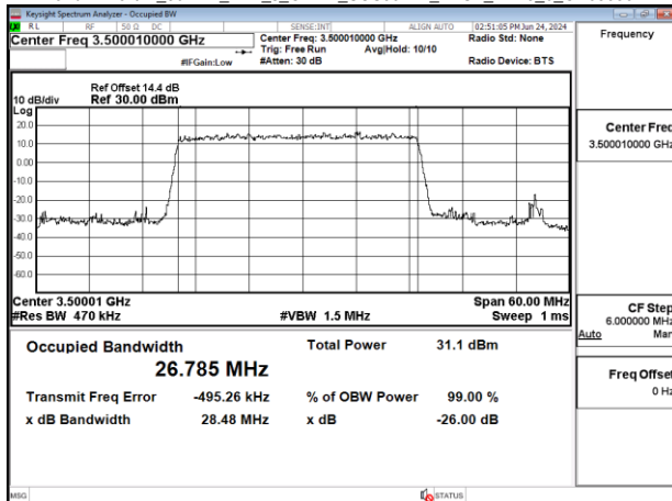
Band77-Part27_30MHz_DFT_s_OFDM_SCS30kHz_BPSK_RB75_0_CH633334
