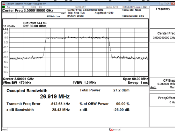
Band77-Part27_30MHz_DFT_s_OFDM_SCS30kHz_256QAM_RB75_0_CH633334
