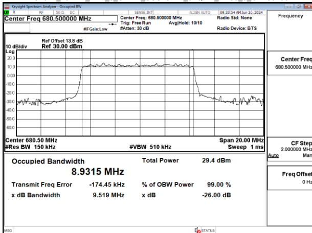
Band71_10MHz_DFT_s_OFDM_SCS15kHz_64QAM_RB50_0_CH136100
