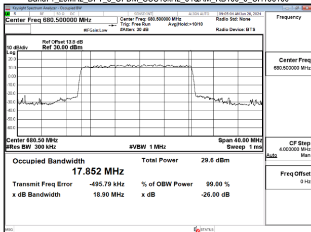
Band71 20MHz DFT_s OFDM SCS15kHz 64QAM RB100_0 CH136100
