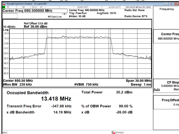
Band71_15MHz_DFT_s_OFDM_SCS15kHz_16QAM_RB75_0_CH136100
