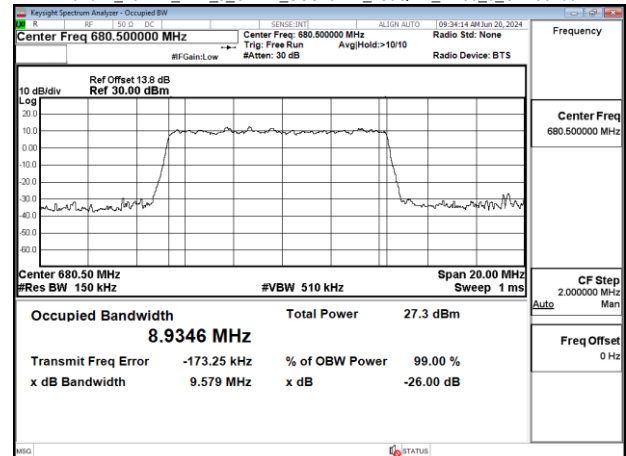
Band71_10MHz_DFT_s_OFDM_SCS15kHz_256QAM_RB50_0_CH136100
