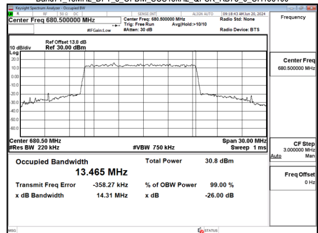
Band71_15MHz_DFT_s_OFDM_SCS15kHz_QPSK_RB75_0_CH136100
