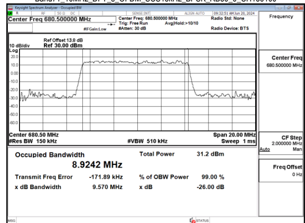
Band71_10MHz_DFT_s_OFDM_SCS15kHz_BPSK_RB50_0_CH136100
