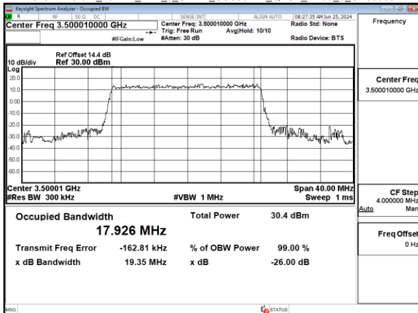
Band7-Part27_20MHz_DFT_s_OFDM_SCS30kHz_QPSK_RB50_0_CH633334
