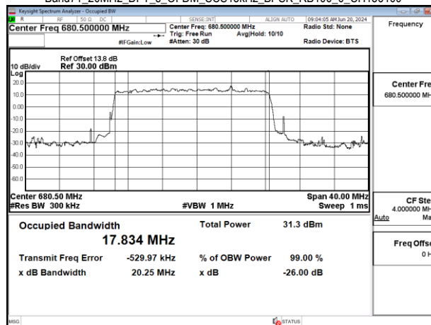
Band71_20MHz_DFT_s_OFDM_SCS15kHz_BPSK_RB100_0_CH136100
