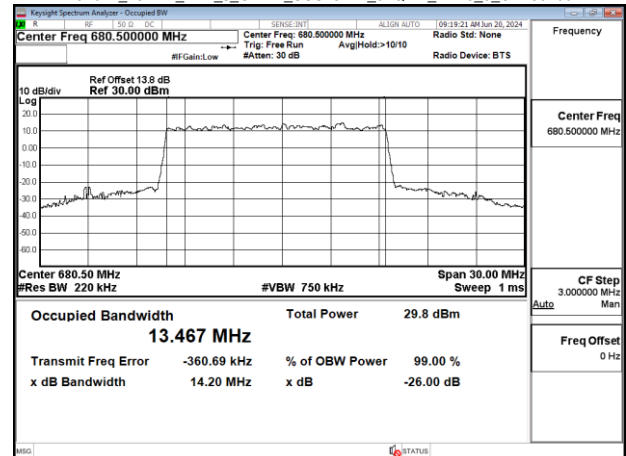
Band71_15MHz_DFT_s_OFDM_SCS15kHz_64QAM_RB75_0_CH136100
