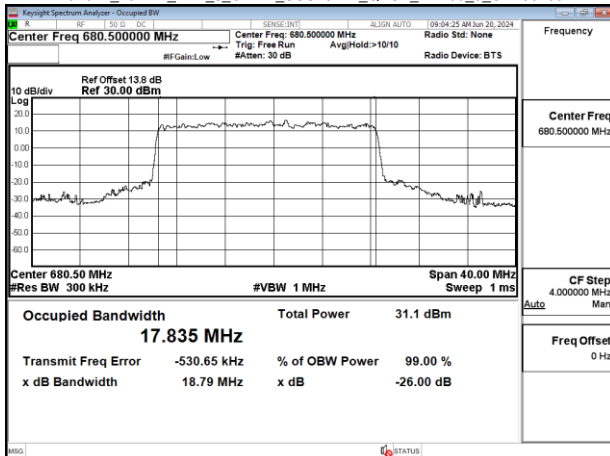
Band71 20MHz DFT s_OFDM_SCS15kHz QPSK_RB100_0_CH136100
