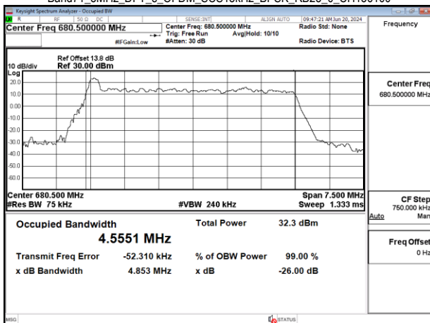
Band71 5MHz DFT s_OFDM_SCS15kHz BPSK_RB25_0_CH136100
