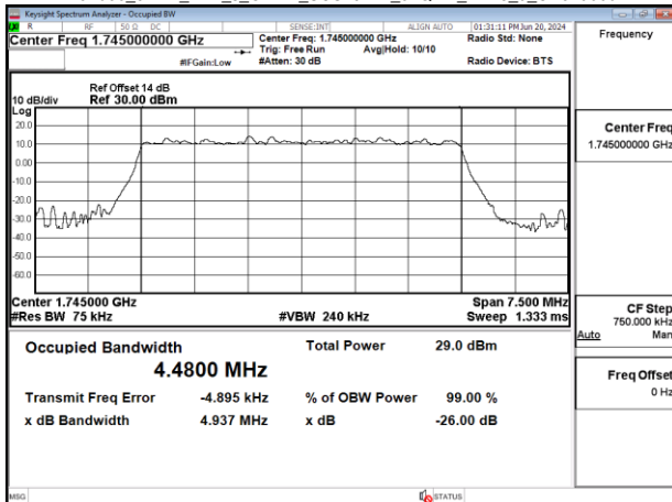
Band66_5MHz_DFT_s_OFDM_SCS15kHz_64QAM_RB25_0_CH349000
