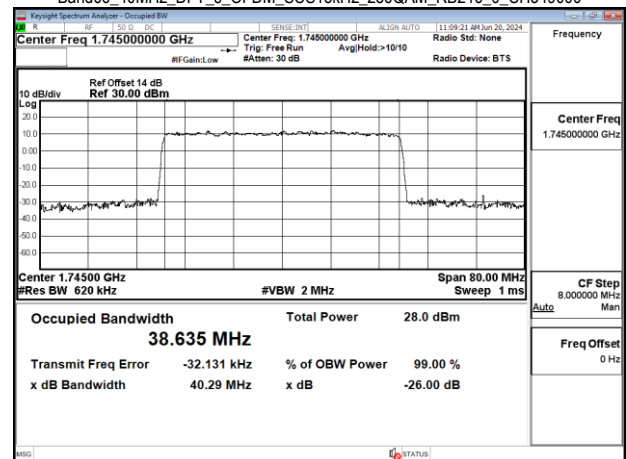
Band66 40MHz DFT s OFDM SCS15kHz 256QAM RB216 0 CH349000
