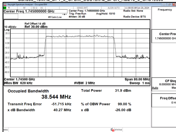
Band66_40MHz_DFT_s_OFDM_SCS15kHz_BPSK_RB216_0_CH349000
