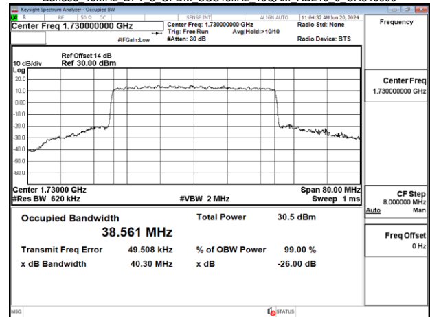
Band66 40MHz DFT s_OFDM_SCS15kHz_16QAM_RB216_0_CH349000
