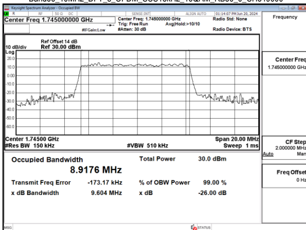
Band66_10MHz_DFT_s_OFDM_SCS15kHz_16QAM_RB50_0_CH349000
