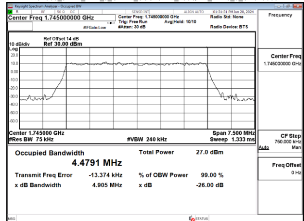
Band66_5MHz_DFT_s_OFDM_SCS15kHz_256QAM_RB25_0_CH349000
