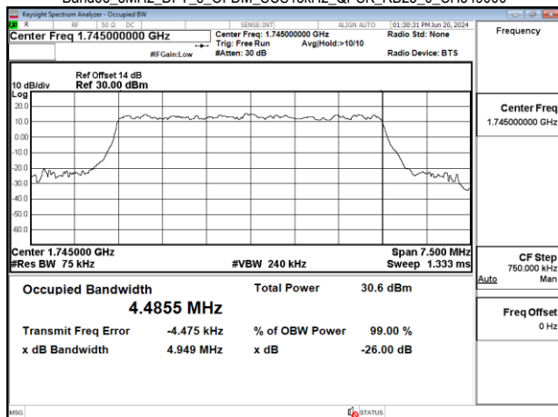
Band66_5MHz_DFT_s_OFDM_SCS15kHz_QPSK_RB25_0_CH349000
