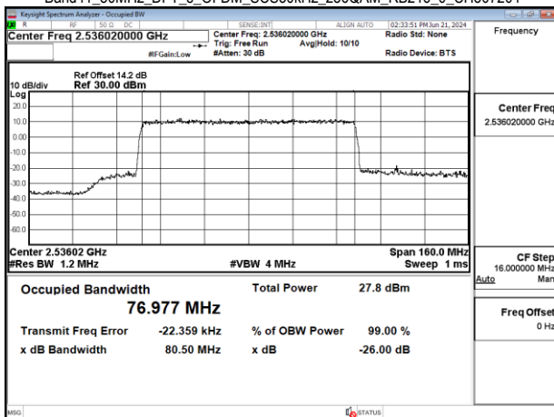
Band41 80MHz DFT s OFDM SCS30kHz 256QAM RB216_0 CH507204
