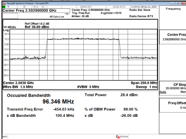
Band41_100MHz_DFT_s_OFDM_SCS30kHz_256QAM_RB270_0_CH518598
