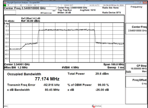
Band41 80MHz DFT s OFDM SCS30kHz 64QAM RB216 0 CH508002
