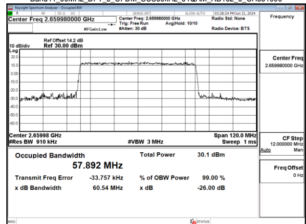
Band41 60MHz DFT s OFDM SCS30kHz 64QAM RB162_0 CH531996
