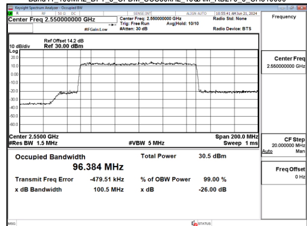
Band41_100MHz_DFT_s_OFDM_SCS30kHz_16QAM_RB270_0_CH510000
