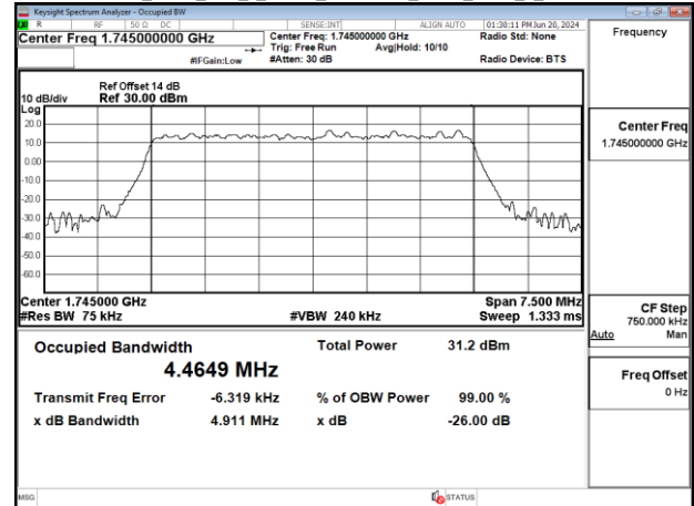
Band66_5MHz_DFT_s_OFDM_SCS15kHz_BPSK_RB25_0_CH349000
