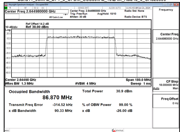
Band41_90MHz_DFT_s_OFDM_SCS30kHz_16QAM_RB243_0_CH528996
