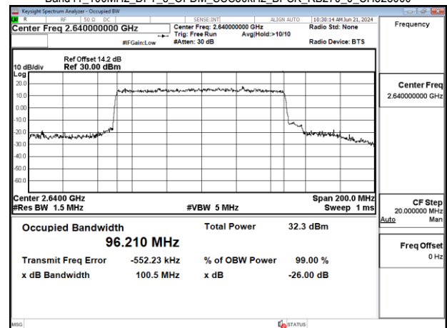
Band41_100MHz_DFT_s_OFDM_SCS30kHz_BPSK_RB270_0_CH528000
