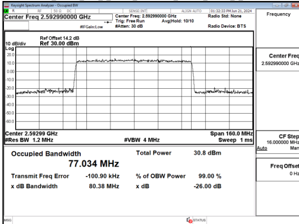
Band41 80MHz DFT s OFDM SCS30kHz 16QAM RB216 0 CH518598
