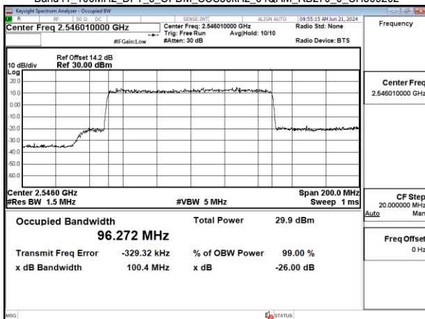
Band41_100MHz_DFT_s_OFDM_SCS30kHz_64QAM_RB270_0_CH509202
