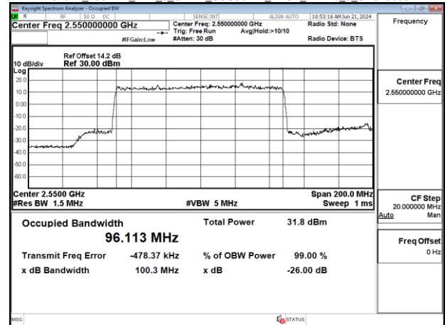
Band41_100MHz_DFT_s_OFDM_SCS30kHz_BPSK_RB270_0_CH518598
