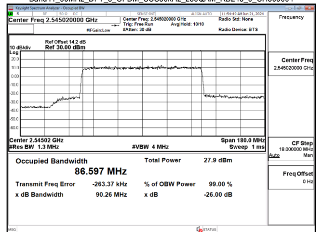
Band41_90MHz_DFT_s_OFDM_SCS30kHz_256QAM_RB243_0_CH509004
