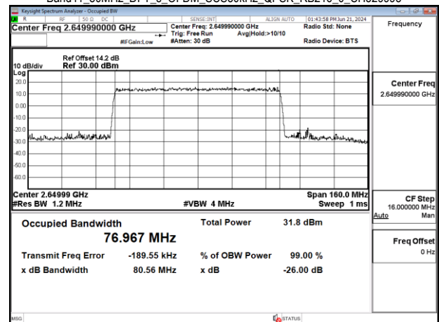
Band41_80MHz_DFT_s_OFDM_SCS30kHz_QPSK_RB216_0_CH529998
