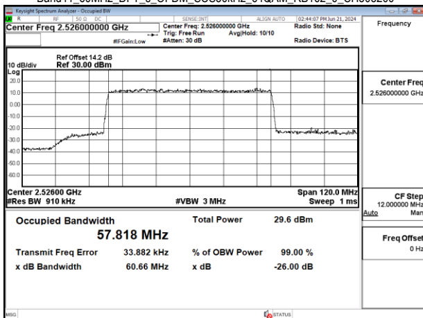
Band41 60MHz DFT s OFDM SCS30kHz 64QAM RB162_0 CH505200
