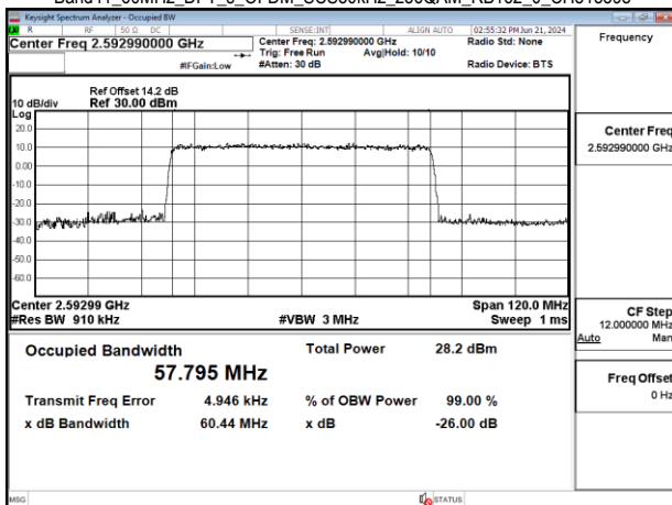
Band41_60MHz_DFT_s_OFDM_SCS30kHz_256QAM_RB162_0_CH518598
