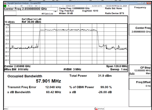
Band41_60MHz_DFT_s_OFDM_SCS30kHz_BPSK_RB162_0_CH531996
