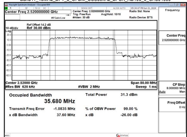
Band41_40MHz_DFT_s_OFDM_SCS30kHz_BPSK_RB100_0_CH504000
