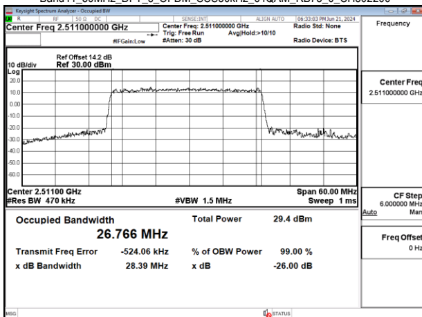
Band41_30MHz_DFT_s_OFDM_SCS30kHz_64QAM_RB75_0_CH502200
