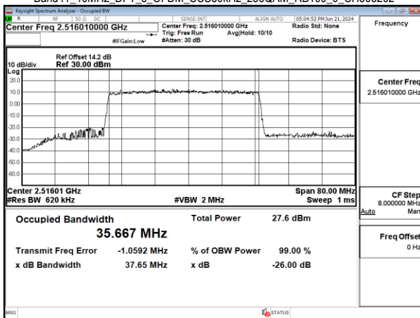
Band41_40MHz_DFT_s_OFDM_SCS30kHz_256QAM_RB100_0_CH503202
