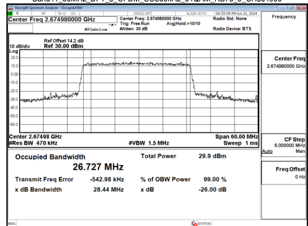
Band41_30MHz_DFT_s_OFDM_SCS30kHz_64QAM_RB75_0_CH534996
