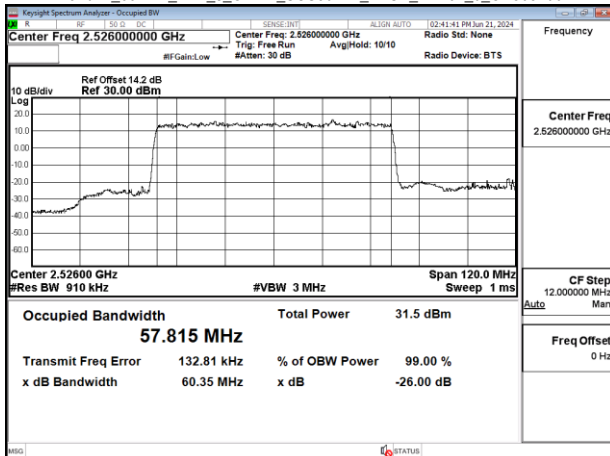
Band41_60MHz_DFT_s_OFDM_SCS30kHz_BPSK_RB162_0_CH505200
