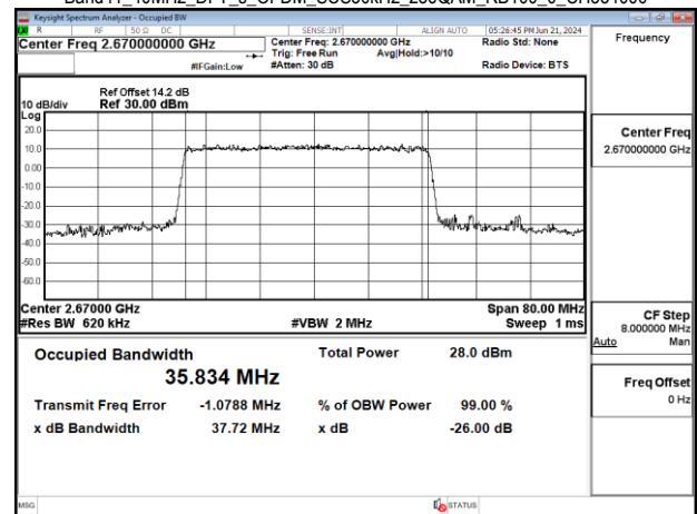
Band41_40MHz_DFT_s_OFDM_SCS30kHz_256QAM_RB100_0_CH534000
