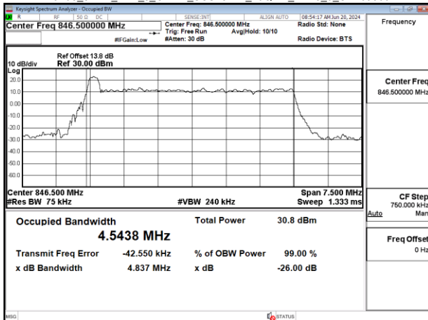
Band5_5MHz_DFT_s_OFDM_SCS15kHz_16QAM_RB25_0_CH169300
