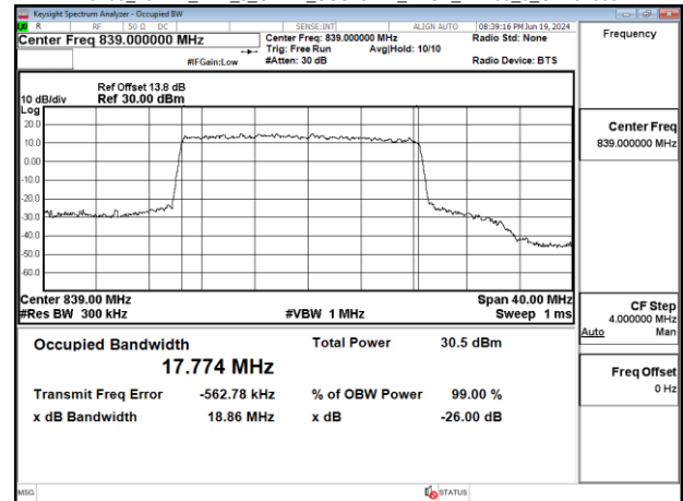
Band5_20MHz_DFT_s_OFDM_SCS15kHz_BPSK_RB100_0_CH167800
