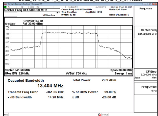
Band5_15MHz_DFT_s_OFDM_SCS15kHz_QPSK_RB75_0_CH168300
