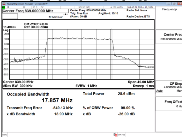
Band5_20MHz_DFT_s_OFDM_SCS15kHz_64QAM_RB100_0_CH167800
