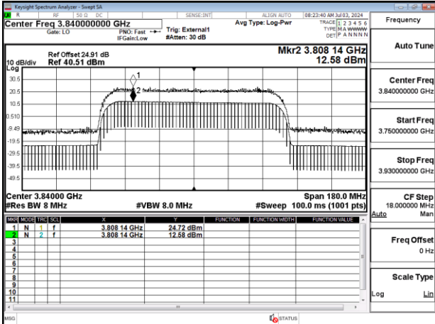
Band77-Part27_90MHz_CP_OFDM_SCS30kHz_256QAM_RB245_0_Chain1_CH656000
