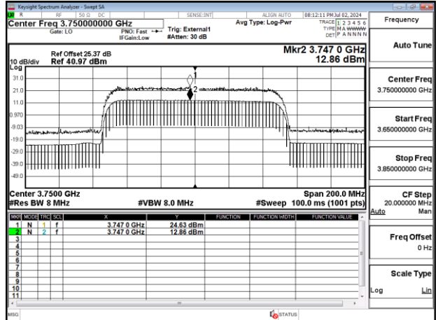
Band77-Part27_100MHz_CP_OFDM_SCS30kHz_256QAM_RB273_0_Chain0_CH650000
