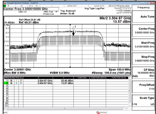
Band77-Part27_90MHz_CP_OFDM_SCS30kHz_256QAM_RB245_0_Chain0_CH633334
