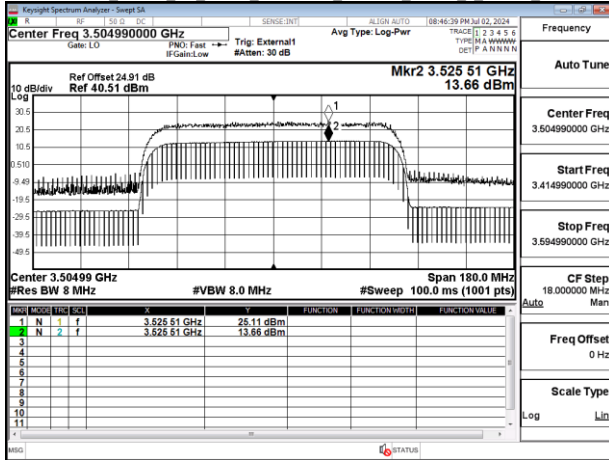
Band77-Part27_90MHz_CP_OFDM_SCS30kHz_256QAM_RB245_0_Chain0_CH649668
