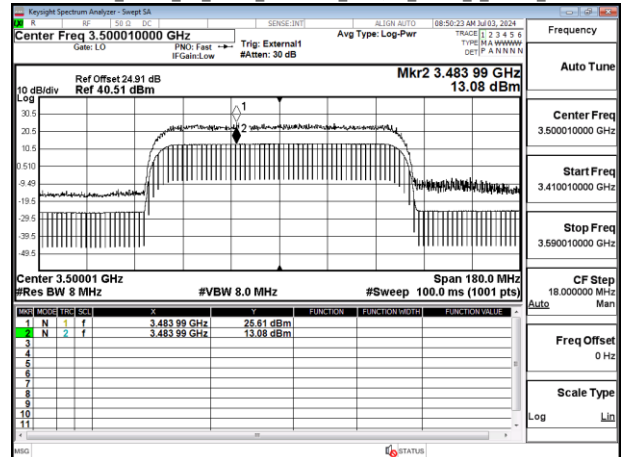
Band77-Part27_90MHz_CP_OFDM_SCS30kHz_256QAM_RB245_0_Chain1_CH633334
