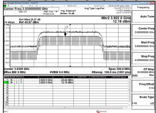
Band77-Part27_100MHz_CP_OFDM_SCS30kHz_256QAM_RB273_0_Chain1_CH662000
