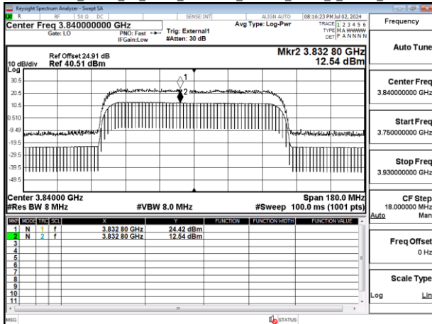
Band77-Part27_90MHz_CP_OFDM_SCS30kHz_256QAM_RB245_0_Chain0_CH656000
