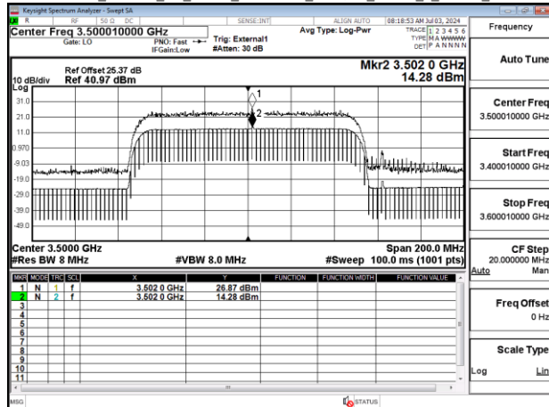
Band77-Part27_100MHz_CP_OFDM_SCS30kHz_256QAM_RB273_0_Chain1_CH633334
