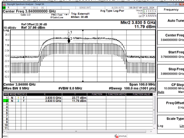
Band77-Part27_50MHz_CP_OFDM_SCS30kHz_256QAM_RB133_0_Chain1_CH656000
