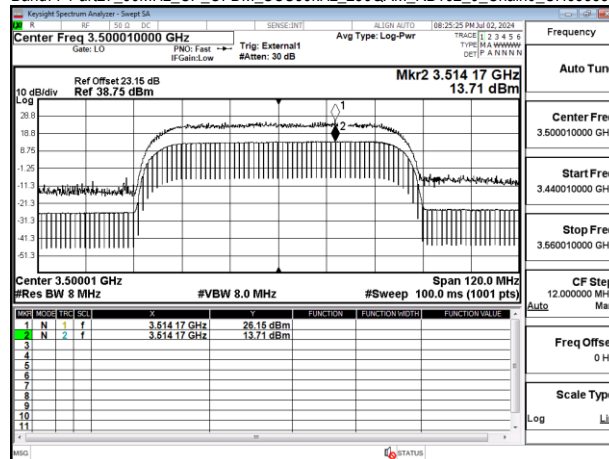
Band77-Part27_60MHz_CP_OFDM_SCS30kHz_256QAM_RB162_0_Chain0_CH633334
