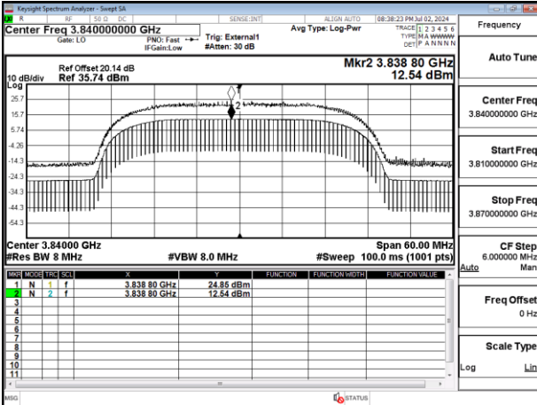
Band77-Part27_30MHz_CP_OFDM_SCS30kHz_256QAM_RB78_0_Chain0_CH656000
