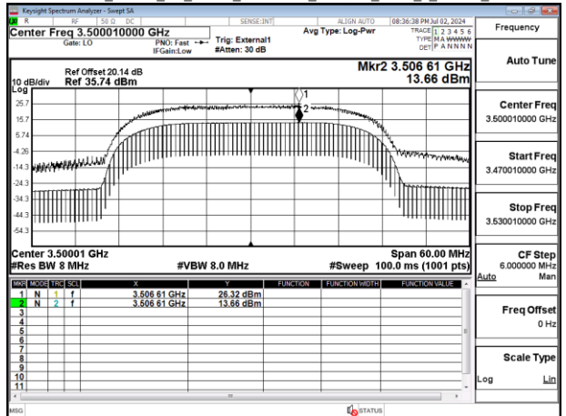
Band77-Part27_30MHz_CP_OFDM_SCS30kHz_256QAM_RB78_0_Chain0_CH633334
