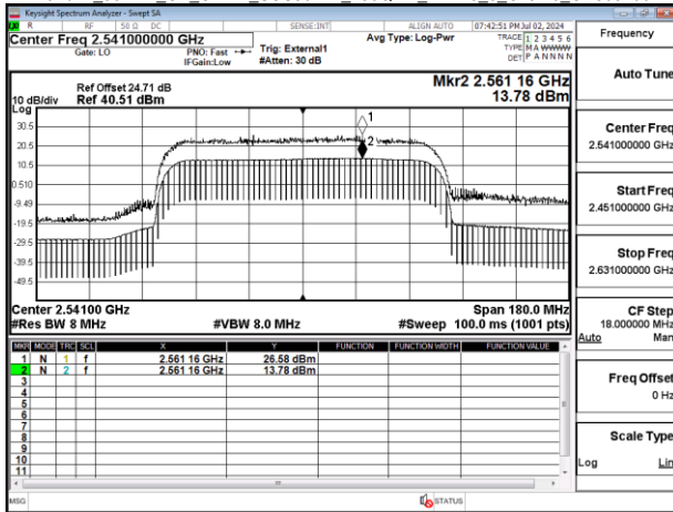
Band41_90MHz_CP_OFDM_SCS30kHz_256QAM_RB245_0_Chain0_CH509004
