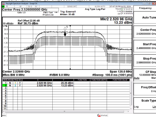
Band41_60MHz_CP_OFDM_SCS30kHz_256QAM_RB162_0_Chain0_CH505200
