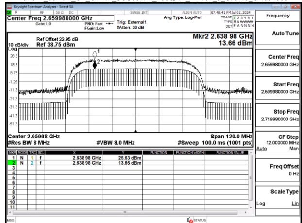
Band41_60MHz_CP_OFDM_SCS30kHz_256QAM_RB162_0_Chain0_CH531996
