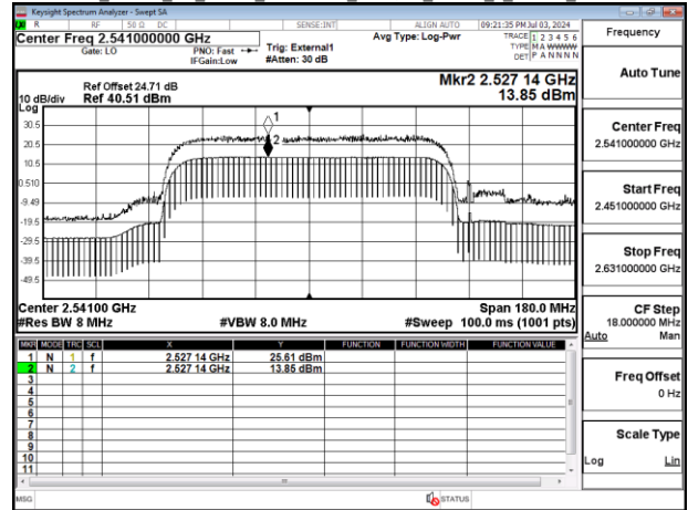
Band41_90MHz_CP_OFDM_SCS30kHz_256QAM_RB245_0_Chain1_CH509004
