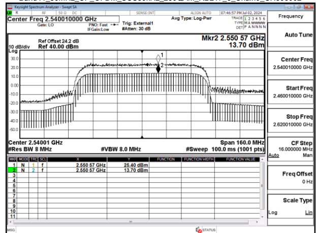
Band41_80MHz_CP_OFDM_SCS30kHz_256QAM_RB217_0_Chain0_CH508002
