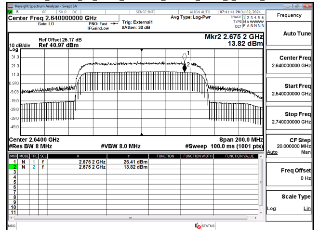
Band41 100MHz CP OFDM SCS30kHz 256QAM RB273 0 Chain0 CH528000
