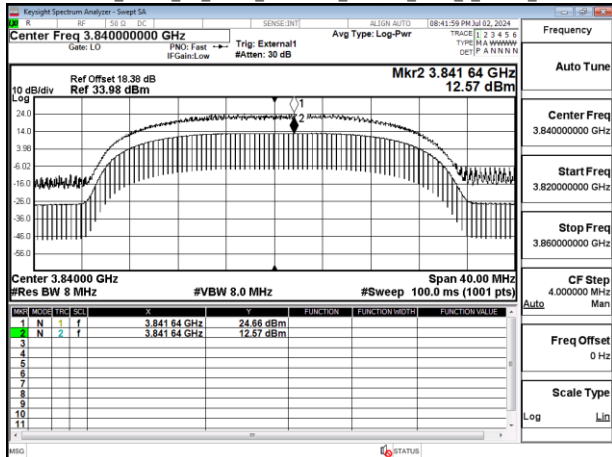
Band77-Part27_20MHz_CP_OFDM_SCS30kHz_256QAM_RB51_0_Chain0_CH656000
