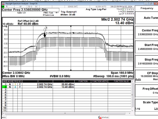
Band41_80MHz_CP_OFDM_SCS30kHz 256QAM_RB217_0_Chain1_CH507204
