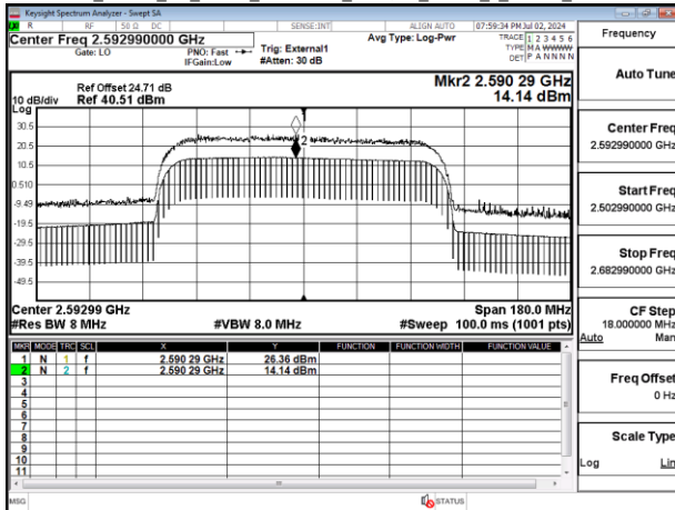
Band41_90MHz_CP_OFDM_SCS30kHz_256QAM_RB245_0_Chain0_CH518598
