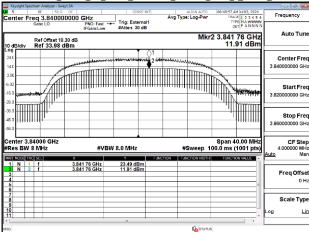
Band77-Part27_20MHz_CP_OFDM_SCS30kHz_256QAM_RB51_0_Chain1_CH656000
