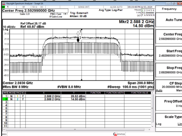
Band41_100MHz_CP_OFDM_SCS30kHz_256QAM_RB273_0_Chain1_CH518598
