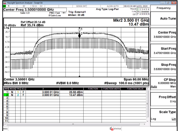
Band77-Part27_30MHz_CP_OFDM_SCS30kHz_256QAM_RB78_0_Chain1_CH633334
