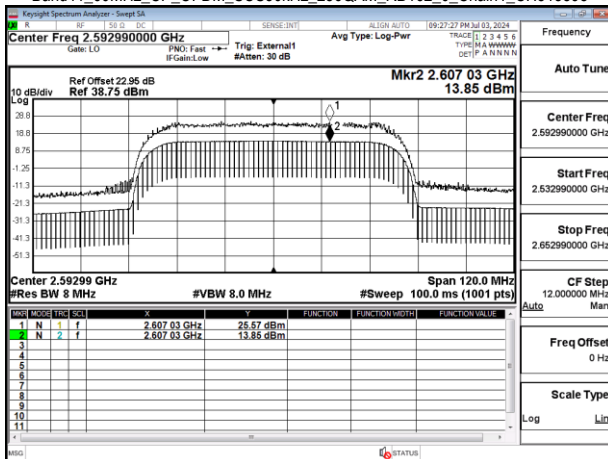
Band41_60MHz_CP_OFDM_SCS30kHz_256QAM_RB162_0_Chain1_CH518598
