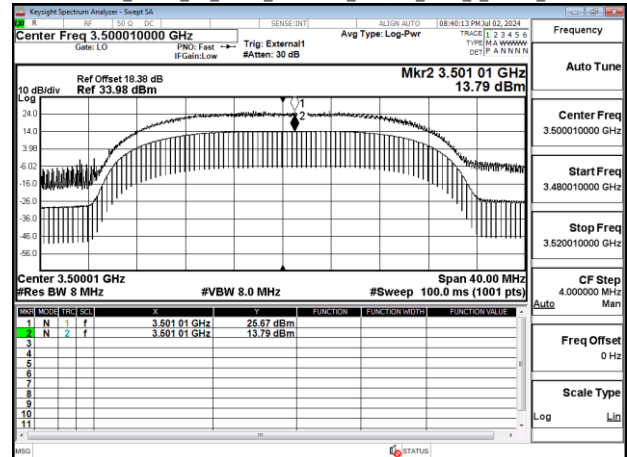
Band77-Part27_20MHz_CP_OFDM_SCS30kHz_256QAM_RB51_0_Chain0_CH633334
