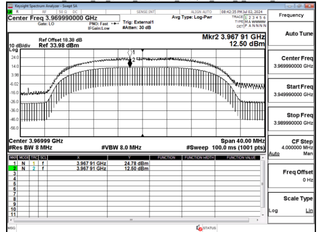
Band77-Part27_20MHz_CP_OFDM_SCS30kHz_256QAM_RB51_0_Chain1_CH630668
