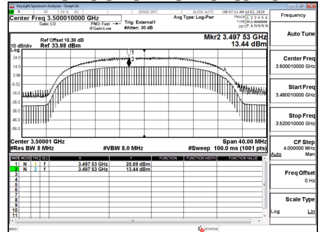
Band77-Part27_20MHz_CP_OFDM_SCS30kHz_256QAM_RB51_0_Chain1_CH633334
