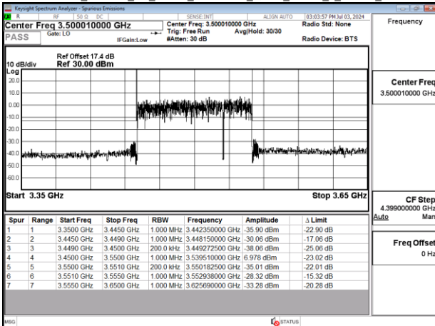
Band77-Part27_100MHz_CP_OFDM_SCS30kHz_QPSK_RB273_0_Chain0_CH633334
