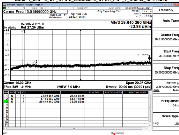
Band41_50MHz_CP_OFDM_SCS30kHz_QPSK_RB1_1_Chain0_CH518598
