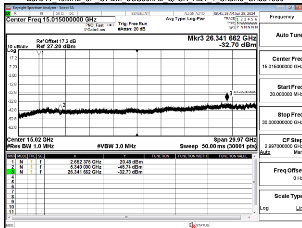
Band41 40MHz CP_OFDM_SCS30kHz_QPSK_RB1_1_Chain0_CH534000
