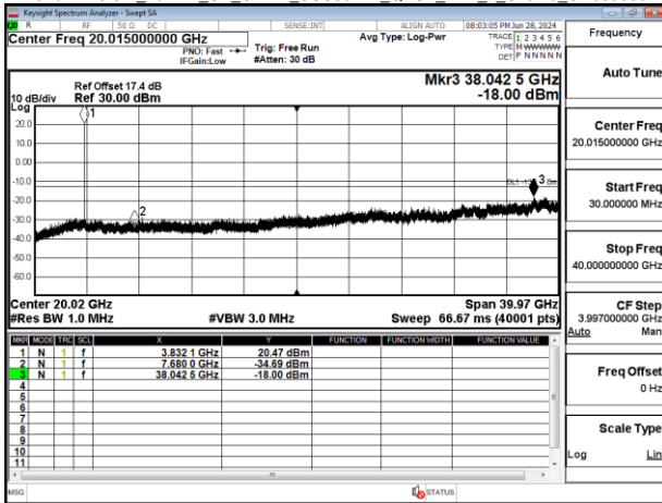
Band77-Part27_20MHz_CP_OFDM_SCS30kHz_QPSK_RB1_1_Chain0_CH664666
