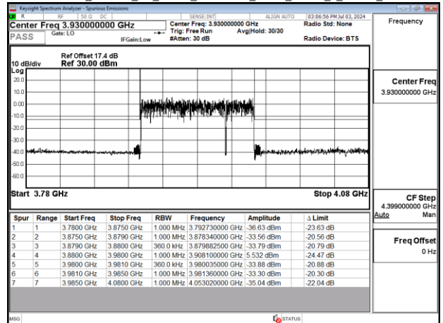
Band77-Part27_100MHz_CP_OFDM_SCS30kHz_QPSK_RB273_0_Chain0_CH662000
