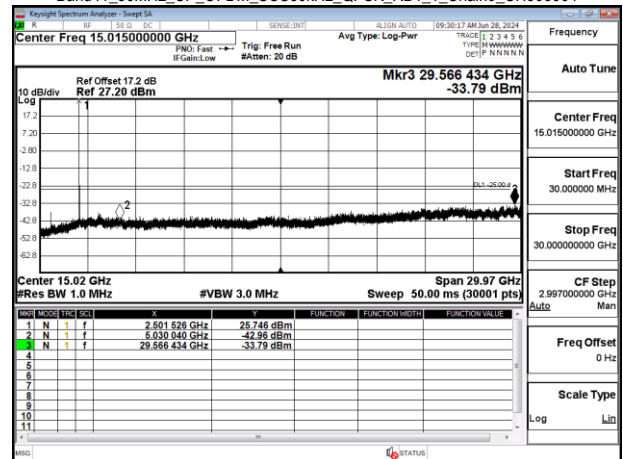
Band41 30MHz CP_OFDM_SCS30kHz_QPSK_RB1_1_Chain0_CH503004
