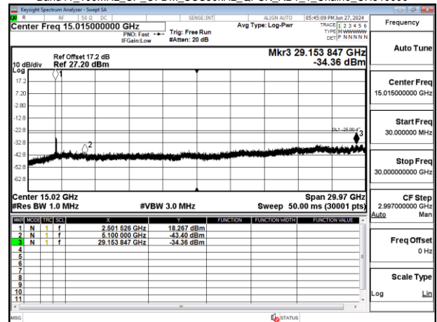
Band41_100MHz_CP_OFDM_SCS30kHz_QPSK_RB1_1_Chain0_CH510000
