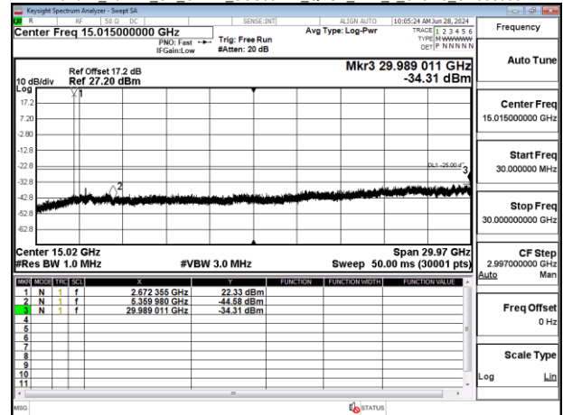
Band41 30MHz CP_OFDM_SCS30kHz_QPSK_RB1_1_Chain0_CH502200
