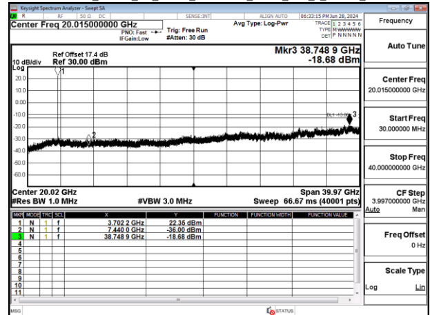
Band77-Part27_40MHz_CP_OFDM_SCS30kHz_QPSK_RB1_1_Chain0_CH648000
