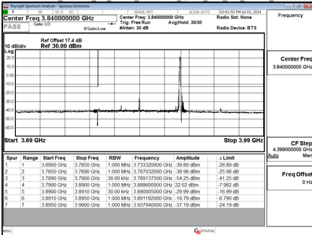
Band77-Part27_100MHz_CP_OFDM_SCS30kHz_QPSK_RB1_272_Chain0_CH662000
