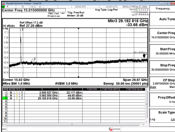
Band41_90MHz_CP_OFDM_SCS30kHz_QPSK_RB1_1_Chain0_CH509004
