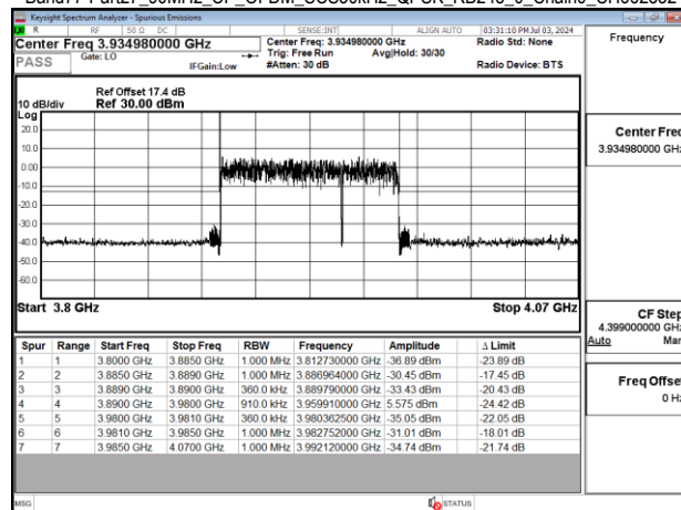
Band77-Part27_90MHz_CP_OFDM_SCS30kHz_QPSK_RB245_0_Chain0_CH623332
