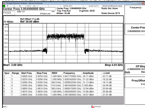
Band77-Part27_50MHz_CP_OFDM_SCS30kHz_QPSK_RB133_0_Chain0_CH663666
