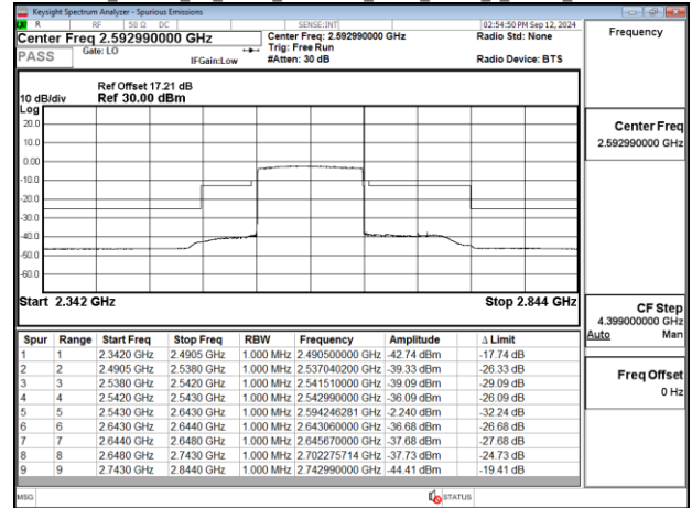
Band41_100MHz_CP_OFDM_SCS30kHz_QPSK_RB273_0_Chain0_CH528000
