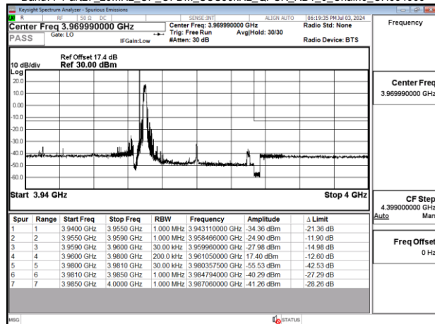
Band77-Part27_20MHz_CP_OFDM_SCS30kHz_QPSK_RB1_0_Chain0_CH664666
