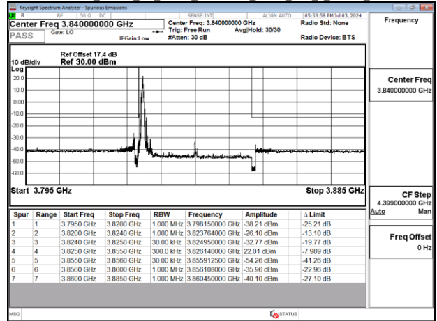
Band77-Part27_30MHz_CP_OFDM_SCS30kHz_QPSK_RB1_0_Chain0_CH664332
