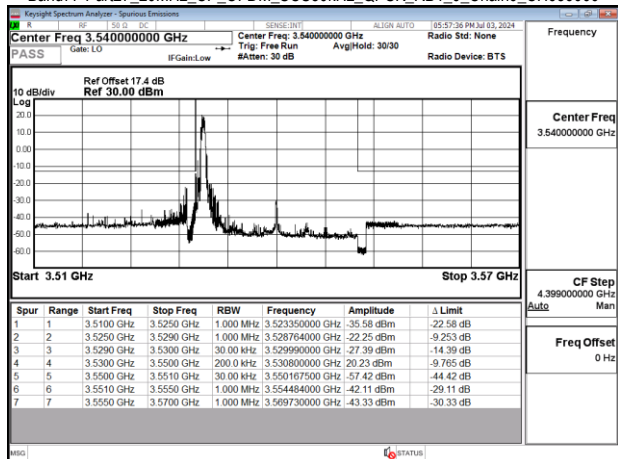
Band77-Part27_20MHz_CP_OFDM_SCS30kHz_QPSK_RB1_0_Chain0_CH636000
