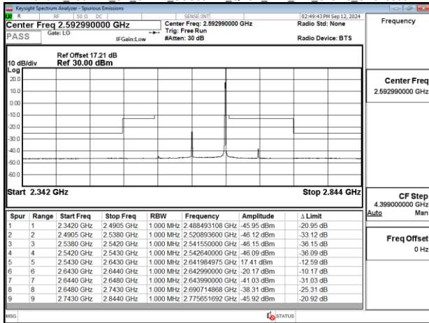
Band41_100MHz_CP_OFDM_SCS30kHz_QPSK_RB1_272_Chain0_CH528000
