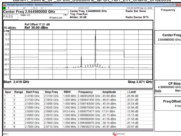
Band41_90MHz_CP_OFDM_SCS30kHz_QPSK_RB245_0_Chain0_CH508200
