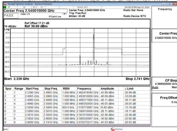
Band41_80MHz_CP_OFDM_SCS30kHz_QPSK_RB1_216_Chain0_CH508002
