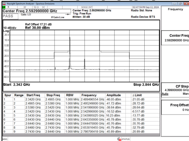
Band41_100MHz_CP_OFDM_SCS30kHz_QPSK_RB1_0_Chain0_CH518598
