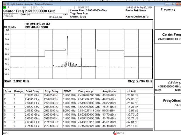
Band41_80MHz_CP_OFDM_SCS30kHz_QPSK_RB1_0_Chain0_CH518598
