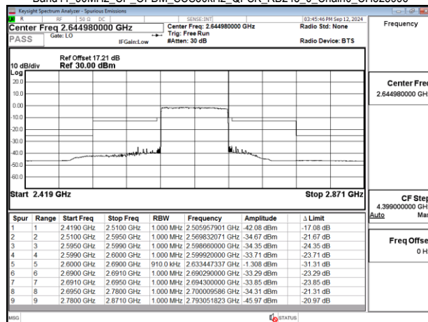
Band41_90MHz_CP_OFDM_SCS30kHz_QPSK_RB245_0_Chain0_CH528996
