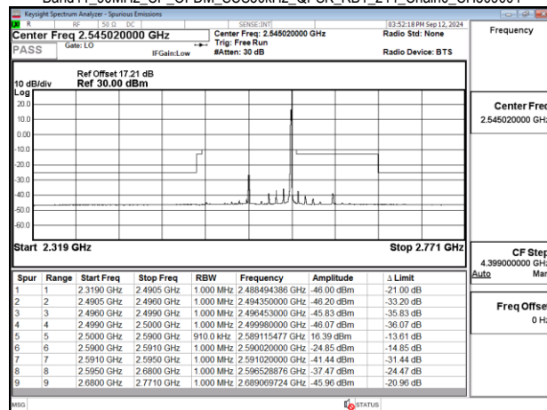
Band41_90MHz_CP_OFDM_SCS30kHz_QPSK_RB1_244_Chain0_CH509004
