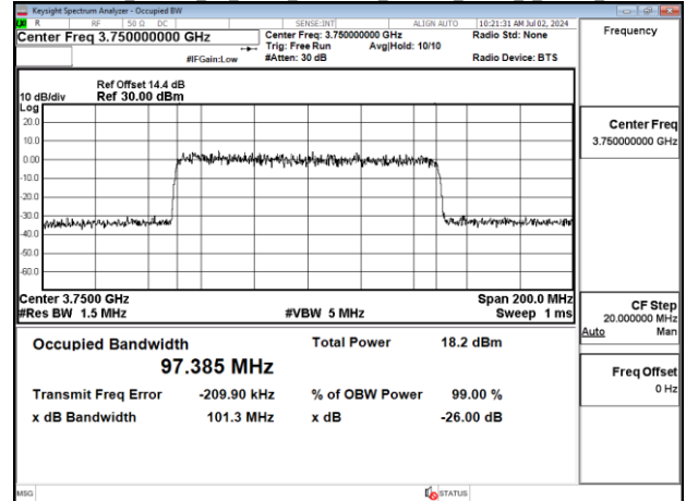
Band77-Part27_100MHz_CP_OFDM_SCS30kHz_256QAM_RB273_0_Chain1_CH650000
