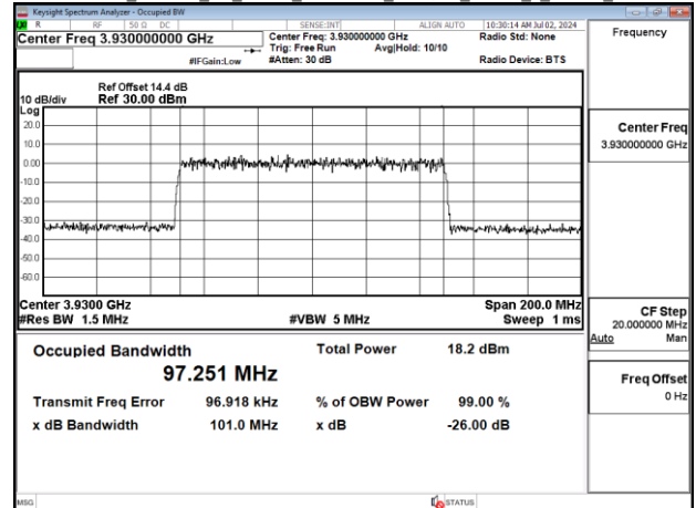
Band77-Part27_100MHz_CP_OFDM_SCS30kHz_256QAM_RB273_0_Chain1_CH662000
