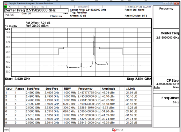
Band41_30MHz_CP_OFDM_SCS30kHz_QPSK_RB1_77_Chain0_CH503004
