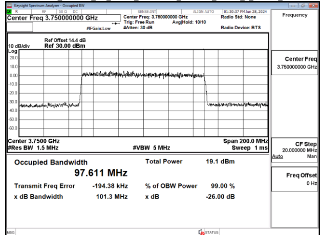
Band77-Part27_100MHz_CP_OFDM_SCS30kHz_256QAM_RB273_0_Chain0_CH650000
