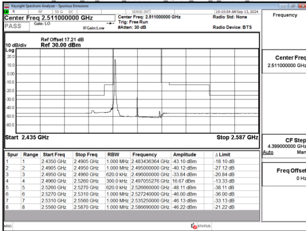
Band41_30MHz_CP_OFDM_SCS30kHz_QPSK_RB1_0_Chain0_CH503004
