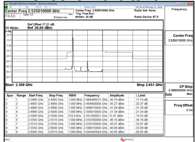
Band41_50MHz_CP_OFDM_SCS30kHz_QPSK_RB1_0_Chain0_CH505002
