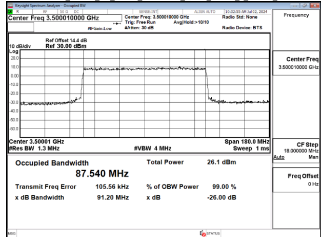
Band77-Part27_90MHz_CP_OFDM_SCS30kHz_QPSK_RB245_0_Chain1_CH633334
