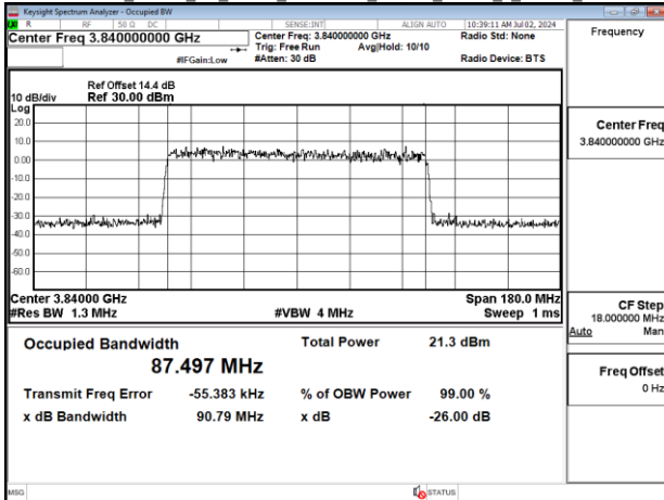
Band77-Part27_90MHz_CP_OFDM_SCS30kHz_64QAM_RB245_0_Chain1_CH656000
