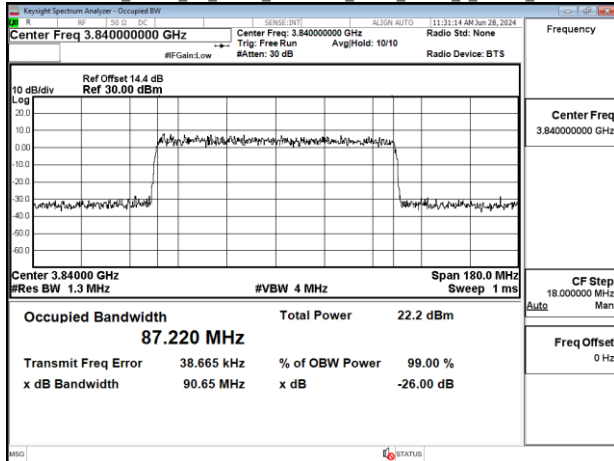
Band77-Part27_90MHz_CP_OFDM_SCS30kHz_QPSK_RB245_0_Chain0_CH656000
