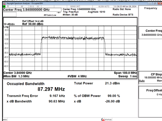
Band77-Part27_90MHz_CP_OFDM_SCS30kHz_64QAM_RB245_0_Chain0_CH656000
