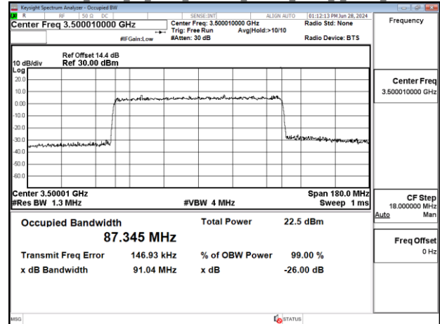
Band77-Part27_90MHz_CP_OFDM_SCS30kHz_256QAM_RB245_0_Chain0_CH633334
