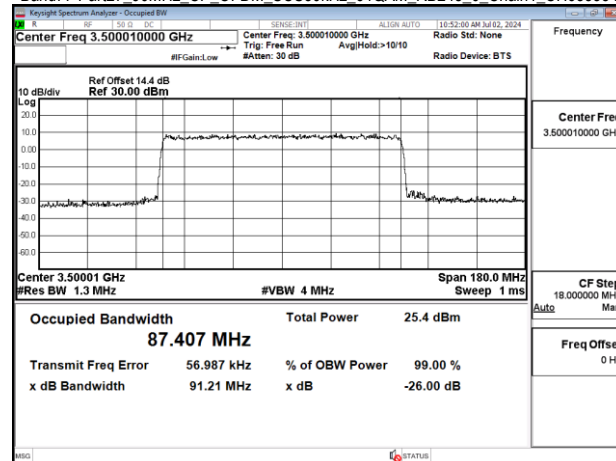
Band77-Part27_90MHz_CP_OFDM_SCS30kHz_64QAM_RB245_0_Chain1_CH633334
