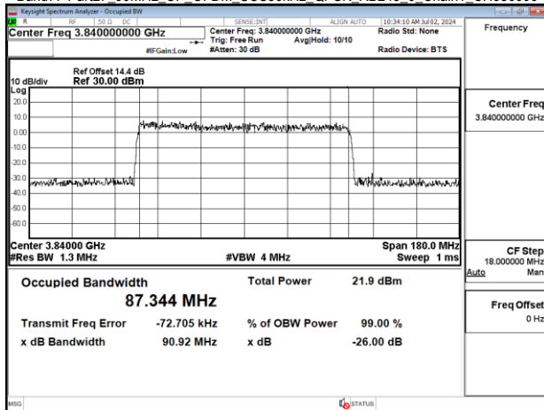
Band77-Part27_90MHz_CP_OFDM_SCS30kHz_QPSK_RB245_0_Chain1_CH656000
