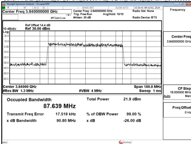
Band77-Part27_90MHz_CP_OFDM_SCS30kHz_16QAM_RB245_0_Chain1_CH656000
