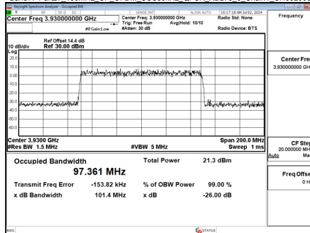
Band77-Part27_100MHz_CP_OFDM_SCS30kHz_QPSK_RB273_0_Chain1_CH662000
