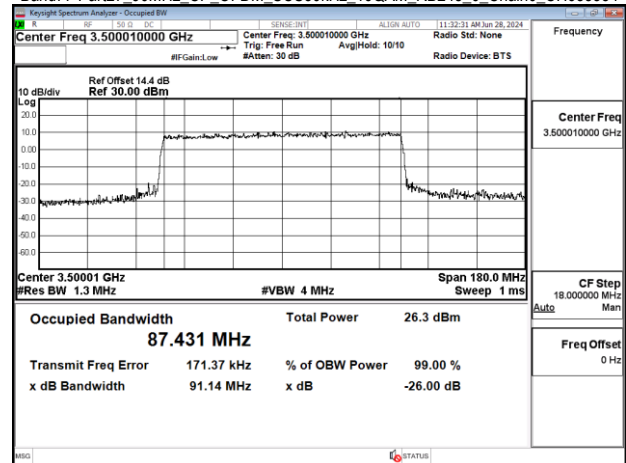
Band77-Part27_90MHz_CP_OFDM_SCS30kHz_16QAM_RB245_0_Chain0_CH633334
