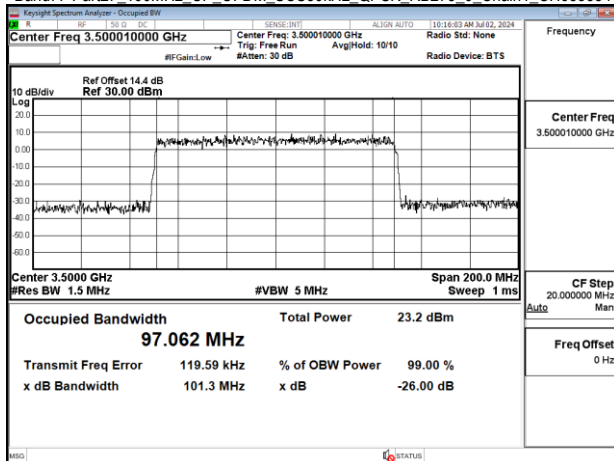
Band77-Part27_100MHz_CP_OFDM_SCS30kHz_QPSK_RB273_0_Chain1_CH633334
