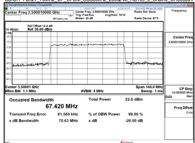
Band77-Part27_70MHz_CP_OFDM_SCS30kHz_256QAM_RB189_0_Chain0_CH633334
