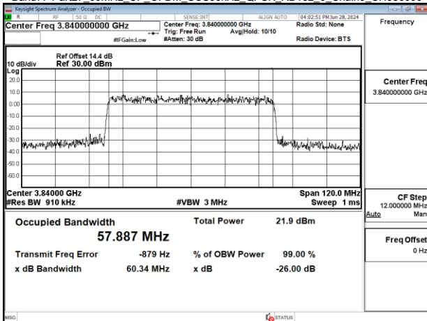
Band77-Part27_60MHz_CP_OFDM_SCS30kHz_QPSK_RB162_0_Chain0_CH656000
