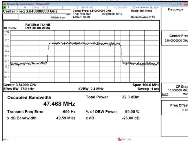
Band77-Part27_50MHz_CP_OFDM_SCS30kHz_QPSK_RB133_0_Chain0_CH656000
