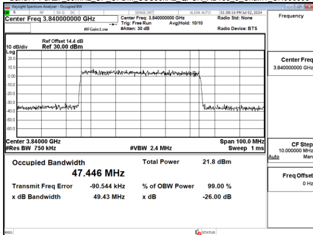
Band77-Part27_50MHz_CP_OFDM_SCS30kHz_QPSK_RB133_0_Chain1_CH656000
