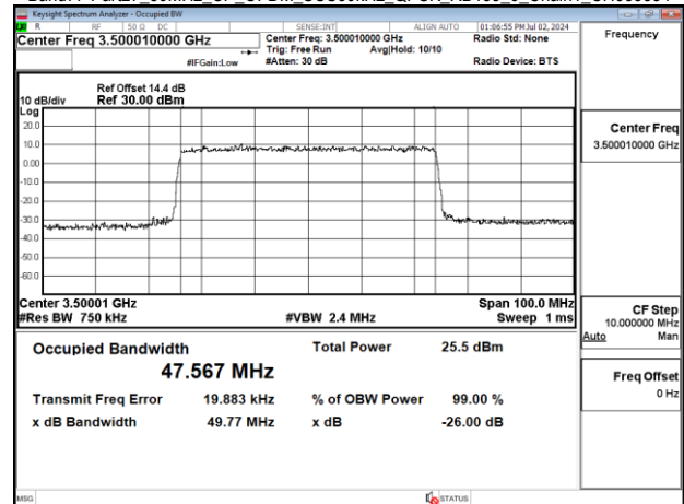
Band77-Part27_50MHz_CP_OFDM_SCS30kHz_QPSK_RB133_0_Chain1_CH633334
