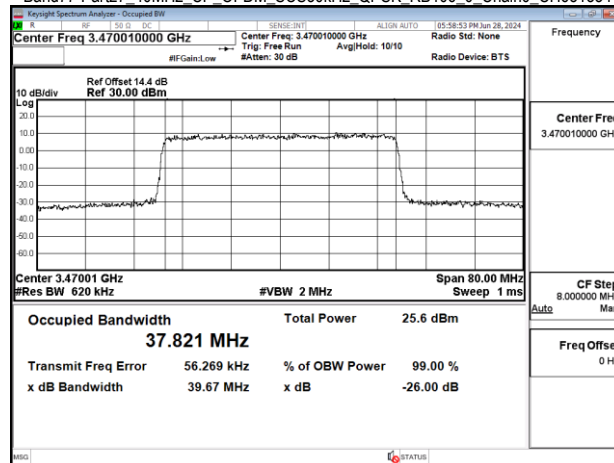
Band77-Part27_40MHz_CP_OFDM_SCS30kHz_QPSK_RB106_0_Chain0_CH633334
