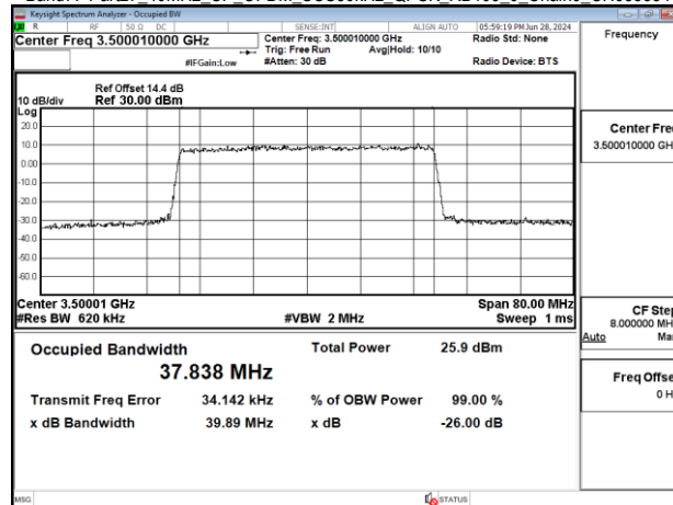
Band77-Part27_40MHz_CP_OFDM_SCS30kHz_QPSK_RB106_0_Chain0_CH633334
