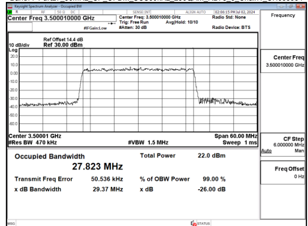
Band77-Part27_30MHz_CP_OFDM_SCS30kHz_256QAM_RB78_0_Chain1_CH633334
