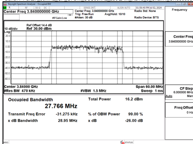
Band77-Part27_30MHz_CP_OFDM_SCS30kHz_256QAM_RB78_0_Chain1_CH656000
