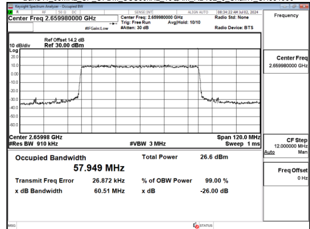
Band41 60MHz CP OFDM, SCS30kHz, 16QAM, RB162_0 Chain1, CH531996
