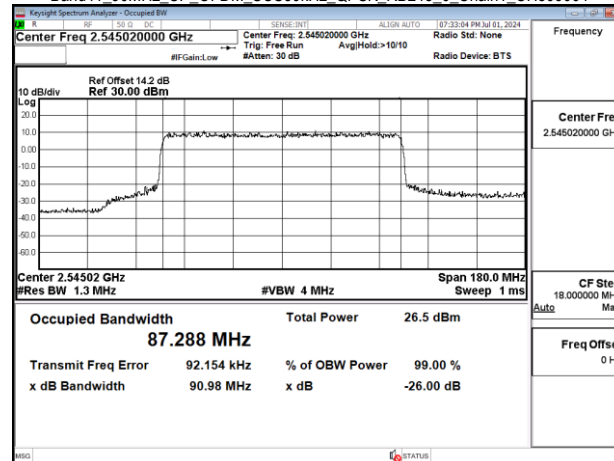
Band41_90MHz_CP_OFDM_SCS30kHz_QPSK_RB245_0_Chain1_CH509004
