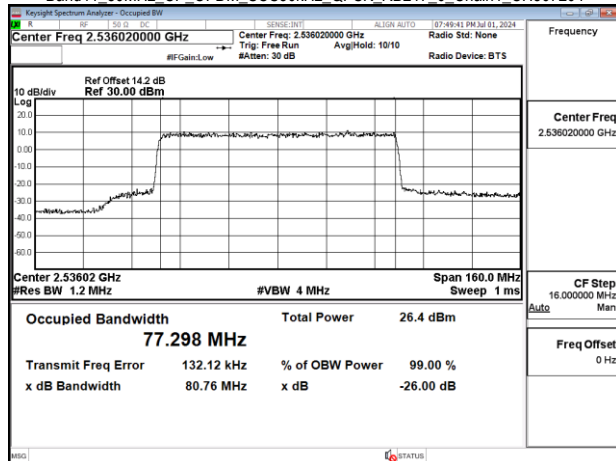
Band41_80MHz_CP_OFDM_SCS30kHz_QPSK_RB217_0_Chain1_CH507204
