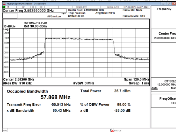
Band41 60MHz CP OFDM SCS30kHz 64QAM RB162_0 Chain0 CH518598
