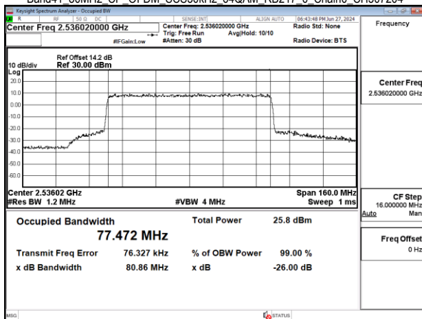
Band41 80MHz CP OFDM SCS30kHz 64QAM RB217 0 Chain0 CH507204
