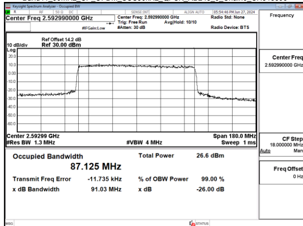
Band41_90MHz_CP_OFDM_SCS30kHz_QPSK_RB245_0_Chain0_CH518598
