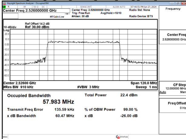
Band41 60MHz CP OFDM_SCS30kHz 256QAM_RB162_0 Chain0_CH505200
