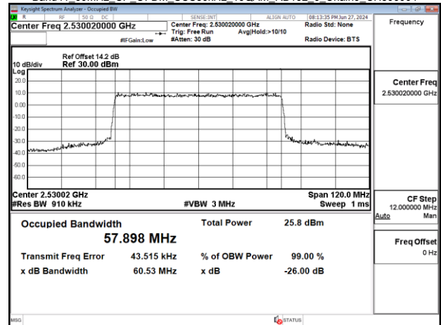
Band41 60MHz CP OFDM SCS30kHz 16QAM RB162_0 Chain0_CH506004
