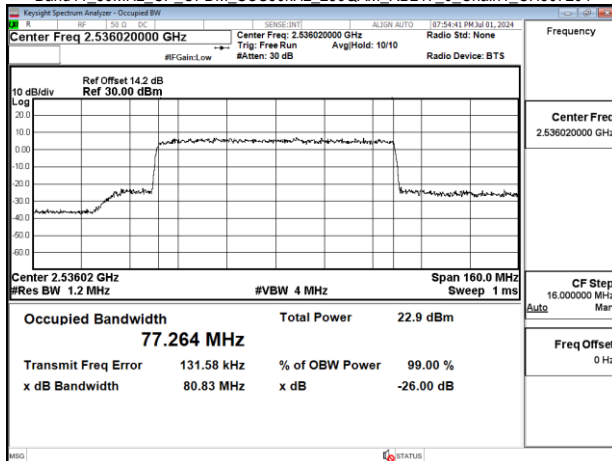
Band41 80MHz CP OFDM_SCS30kHz_256QAM_RB217_0_Chain1_CH507204
