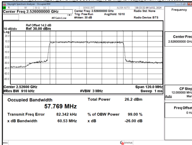
Band41 60MHz CP OFDM, SCS30kHz, 16QAM, RB162_0 Chain1, CH505200
