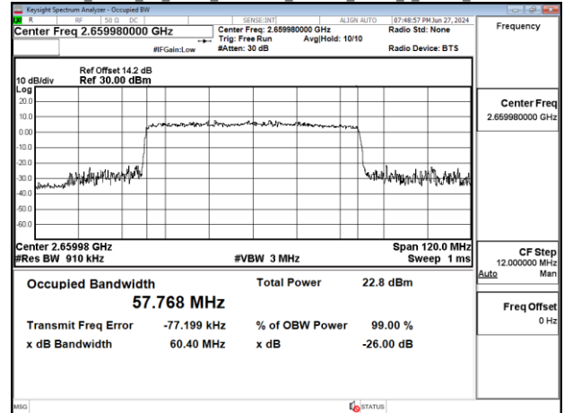
Band41 60MHz CP OFDM_SCS30kHz 256QAM_RB162_0 Chain0_CH531996
