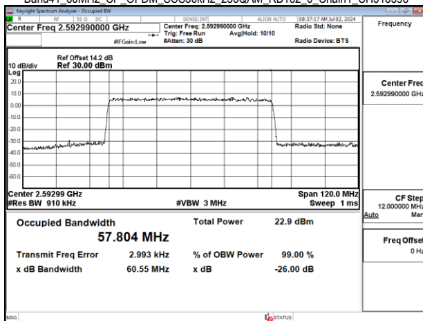
Band41 60MHz CP OFDM_SCS30kHz 256QAM_RB162_0 Chain1_CH518598
