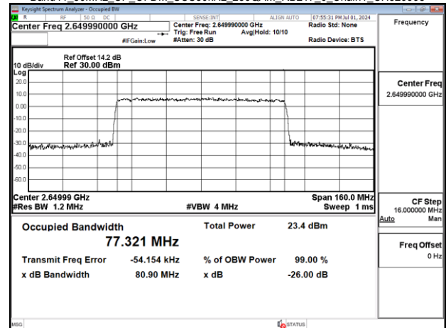
Band41 80MHz CP OFDM_SCS30kHz_256QAM_RB217_0_Chain1_CH529998
