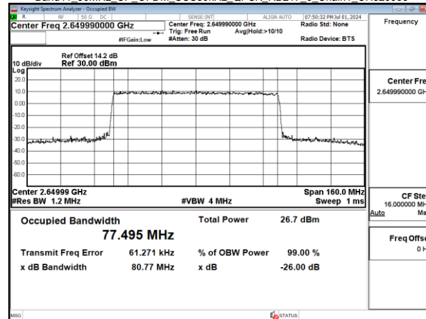
Band41_80MHz_CP_OFDM_SCS30kHz_QPSK_RB217_0_Chain1_CH529998
