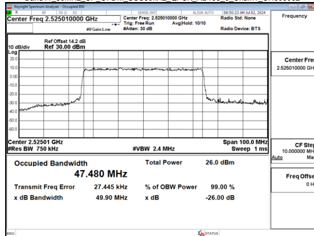
Band41_50MHz_CP_OFDM_SCS30kHz_QPSK_RB133_0_Chain1_CH505002
