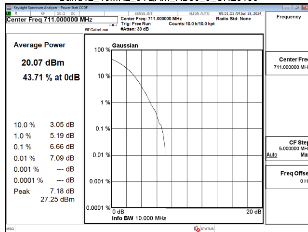
Band12_10MHz_64QAM_RB50_0_CH23130
