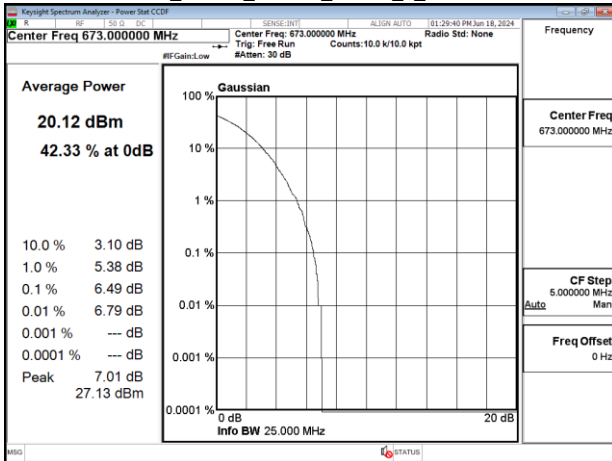
Band71_20MHz_64QAM_RB100_0_CH133222
