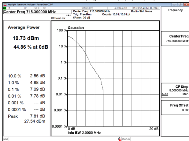
Band12_1.4MHz_64QAM_RB6_0_CH23173
