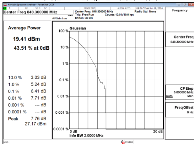
Band5_1.4MHz_64QAM_RB6_0_CH20643
