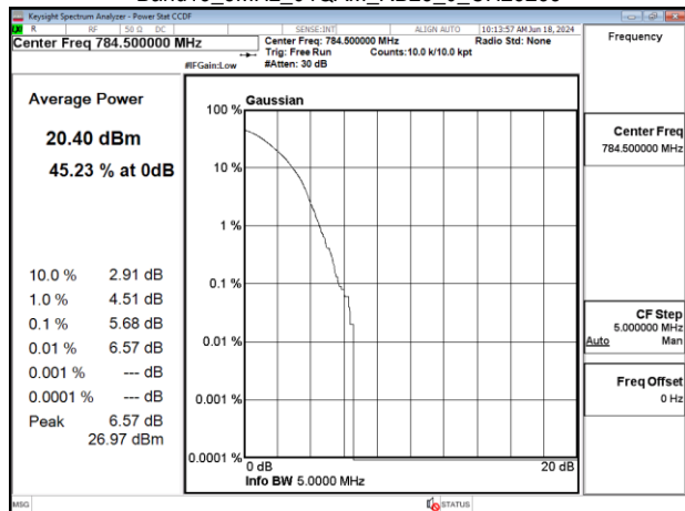
Band13_5MHz_64QAM_RB25_0_CH23255
