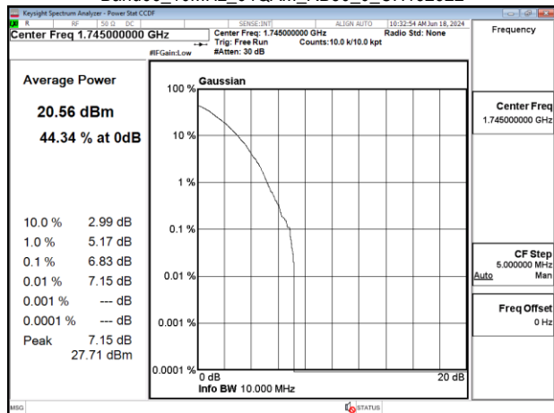
Band66_10MHz_64QAM_RB50_0_CH132322
