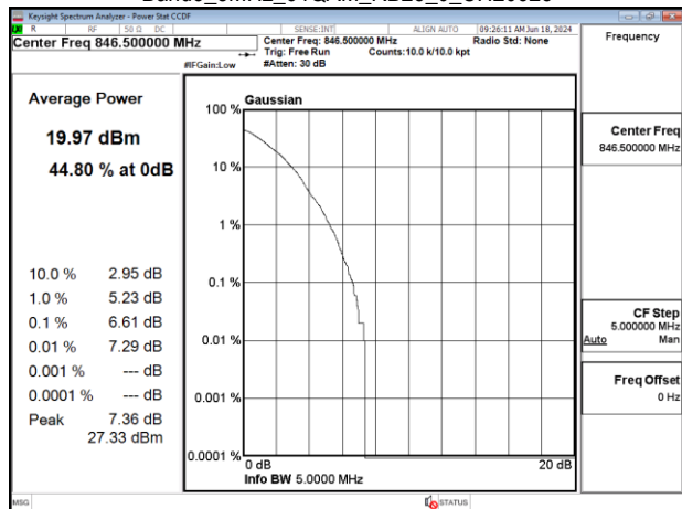
Band5_5MHz_64QAM_RB25_0_CH20625
