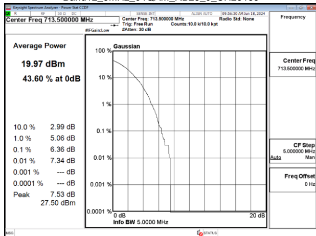
Band12_5MHz_64QAM_RB25_0_CH23155
