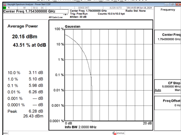
Band4_1.4MHz_64QAM_RB6_0_CH20393
