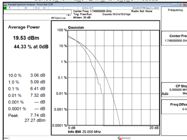
Band66_15MHz_64QAM_RB75_0_CH132322
