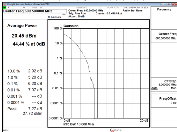
Band71_10MHz_64QAM_RB50_0_CH133297
