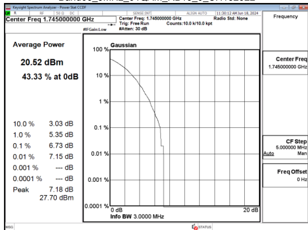
Band66_3MHz_64QAM_RB15_0_CH132322
